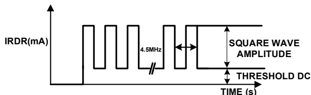
FIGURE 6. TYPICAL EMITTER WAVEFORM AND FEATURES
