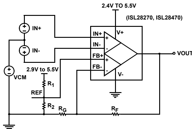
FIGURE 50. GAIN SETTING AND REFERENCE CONNECTION
