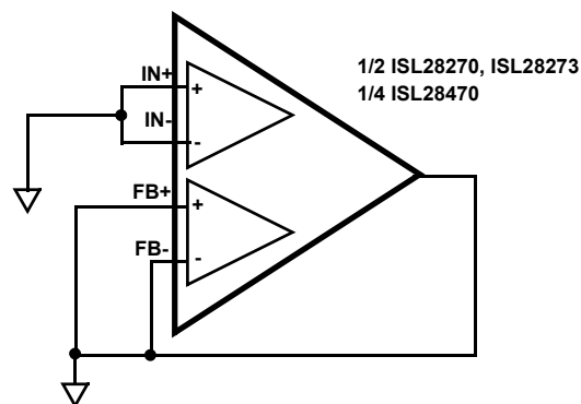
FIGURE 52. PREVENTING OSCILLATIONS IN UNUSED CHANNELS
