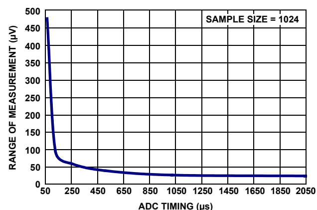
FIGURE 92. AUXILIARY SHUNT STABILITY: RANGE vs ACQUISITION TIME
