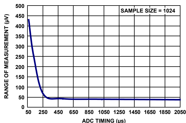
FIGURE 88. PRIMARY SHUNT STABILITY: RANGE vs ACQUISITION TIME
