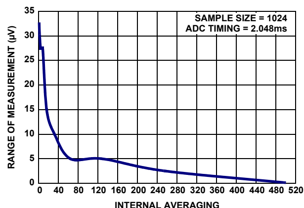
FIGURE 90. PRIMARY SHUNT STABILITY: RANGE vs INTERNAL AVERAGING
