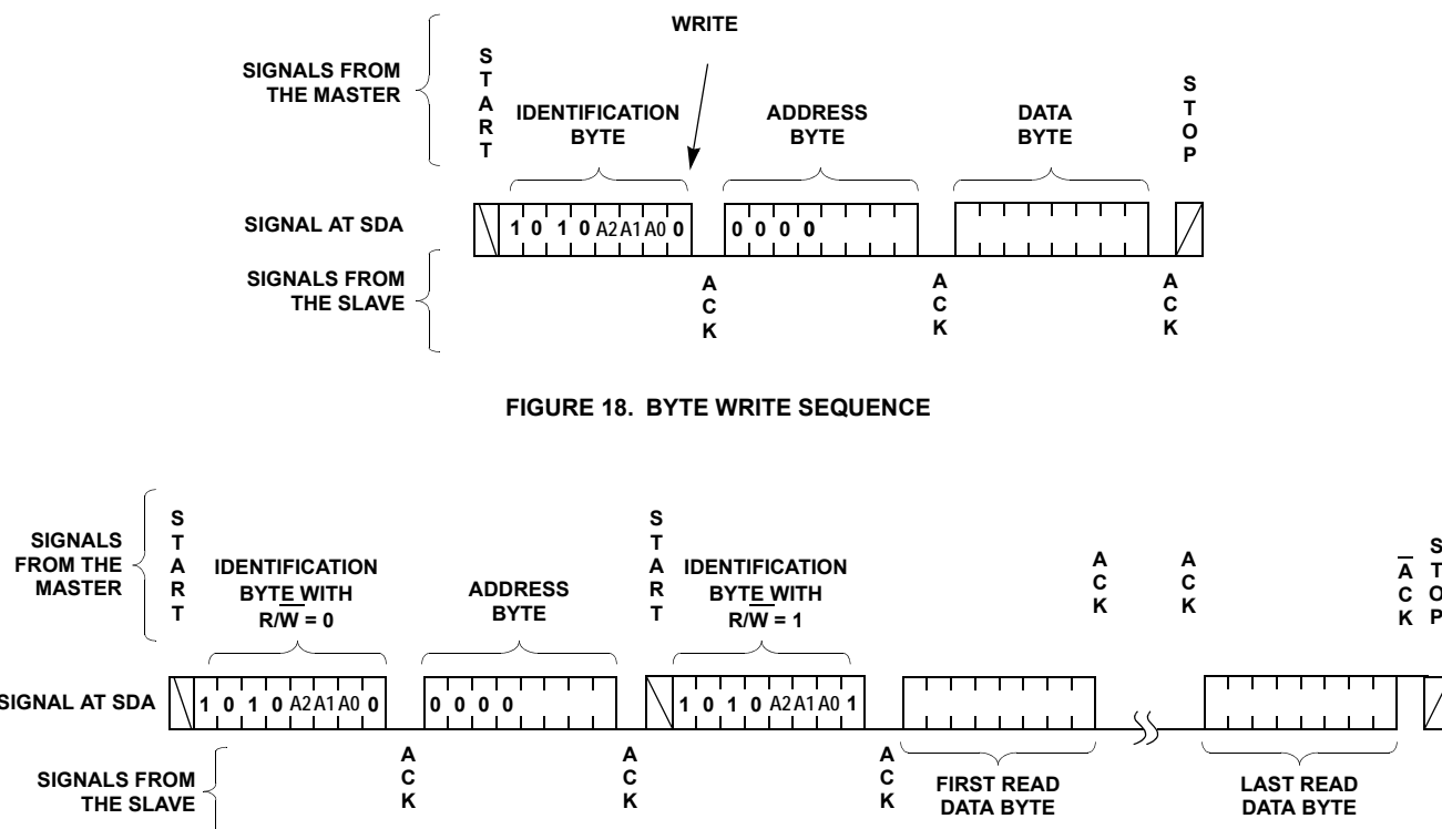
FIGURE 19. READ SEQUENCE
