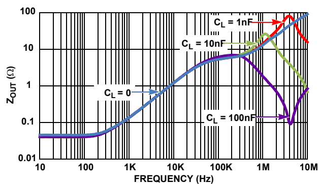
FIGURE 62. Z_{OUT} vs FREQUENCY
