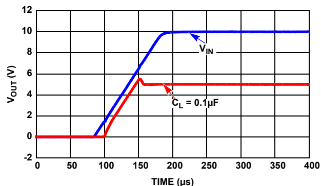
FIGURE 44. TURN-ON TIME WITH 0.1 \mu\text{F}
