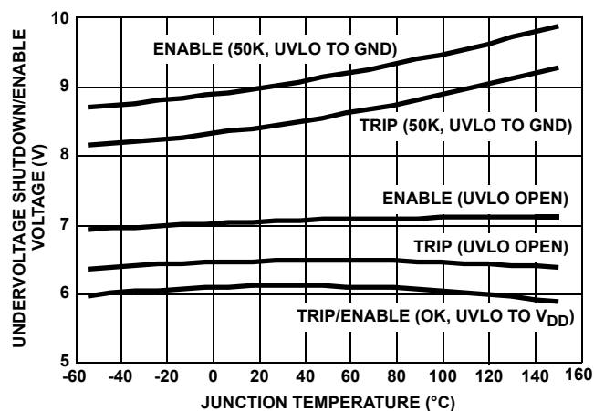
FIGURE 7. UNDERVOLTAGE THRESHOLD
