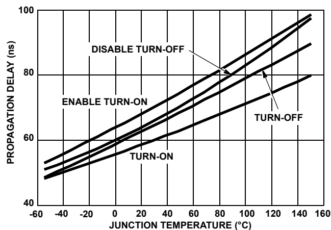
FIGURE 8. PROPAGATION DELAY
