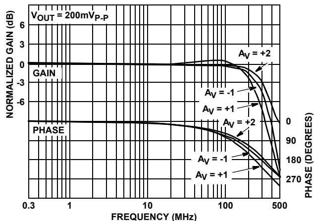
FIGURE 10. FREQUENCY RESPONSE
