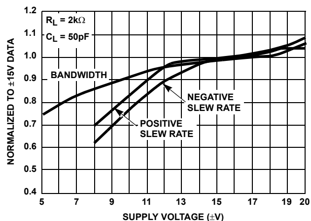
FIGURE 19. NORMALIZED AC PARAMETERS vs SUPPLY VOLTAGE
