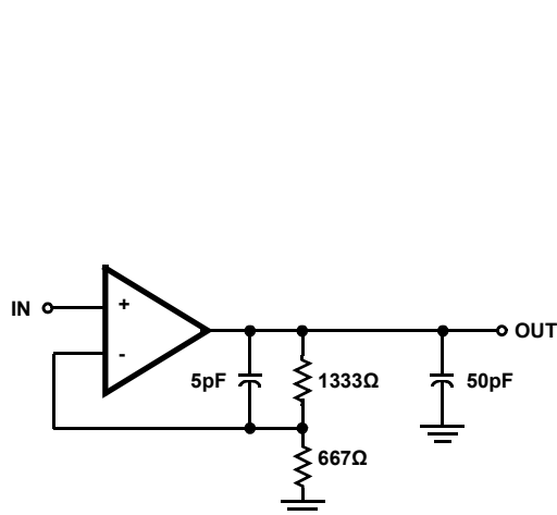
FIGURE 1. SLEW RATE AND SETTLE TIME
