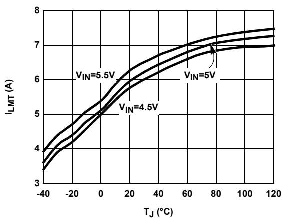
FIGURE 11. CURRENT LIMIT vs T_J
