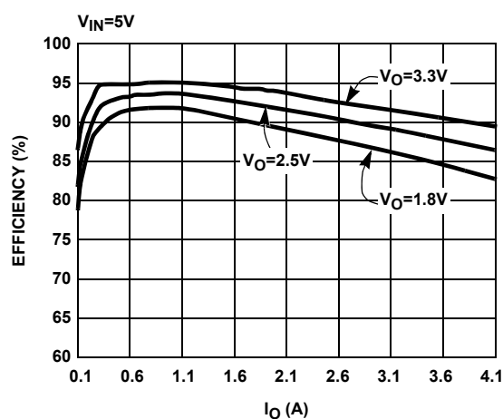
FIGURE 2. EL7564CRE EFFICIENCY
