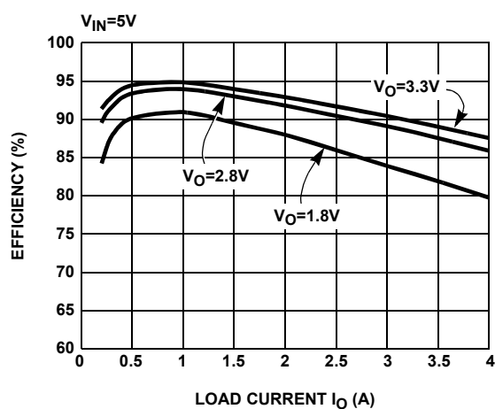
FIGURE 1. EL7564CM EFFICIENCY
