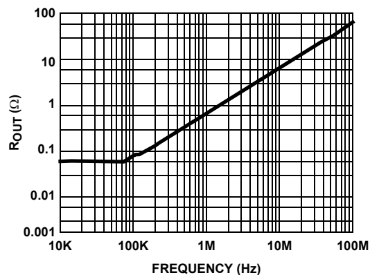
FIGURE 31. CLOSED LOOP OUTPUT IMPEDANCE vs FREQUENCY
