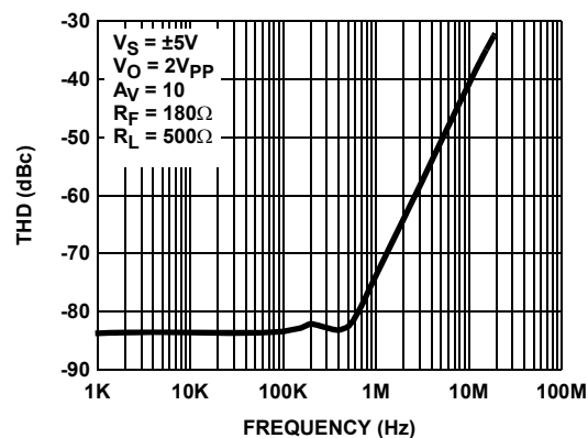
FIGURE 25. TOTAL HARMONIC DISTORTION vs FREQUENCY
