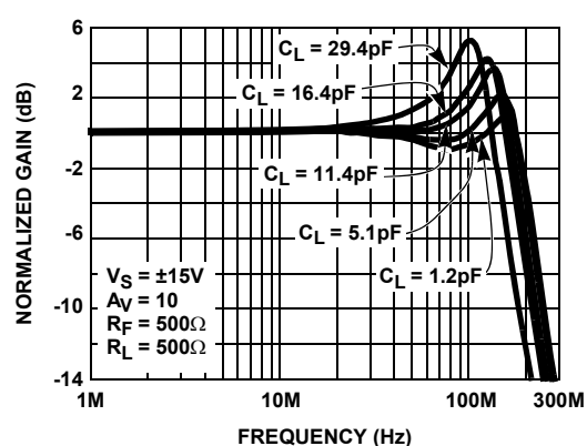
FIGURE 14. INVERTING FREQUENCY RESPONSE FOR VARIOUS C_L
