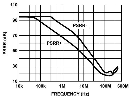
FIGURE 30. PSRR
