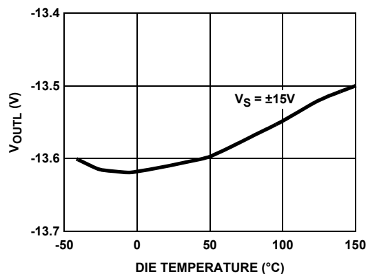
FIGURE 43. NEGATIVE OUTPUT SWING vs TEMPERATURE
