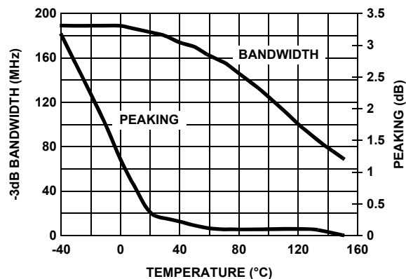
FIGURE 32. BANDWIDTH vs TEMPERATURE
