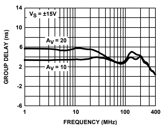
FIGURE 28. GROUP DELAY
