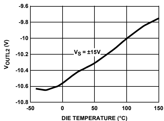
FIGURE 45. NEGATIVE OUTPUT SWING vs TEMPERATURE
