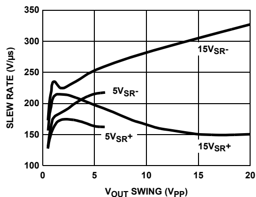
FIGURE 33. SLEW RATE vs SWING
