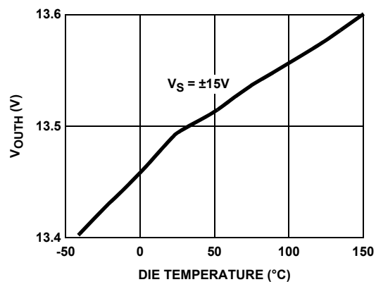
FIGURE 41. POSITIVE OUTPUT SWING vs TEMPERATURE
