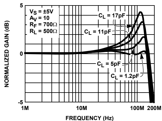
FIGURE 12. NON-INVERTING FREQUENCY RESPONSE FOR VARIOUS C_L
