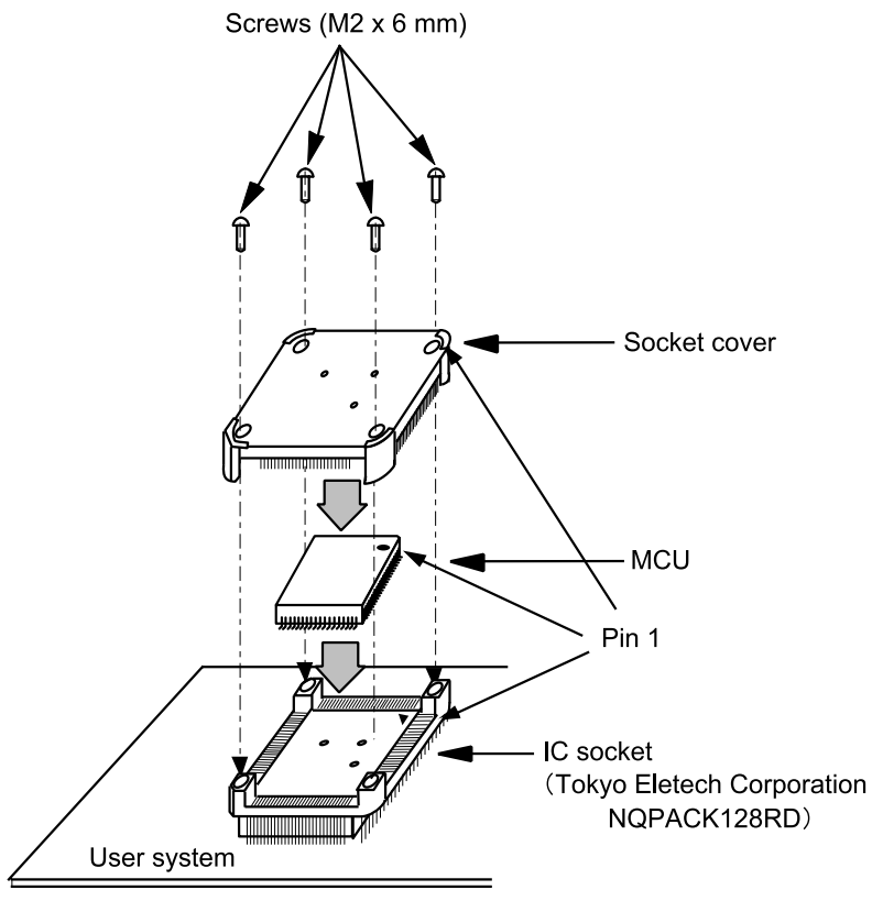
Figure 9 Installing MCU to User System
