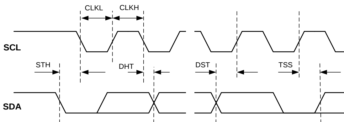
Figure 5. I²C bus timing
