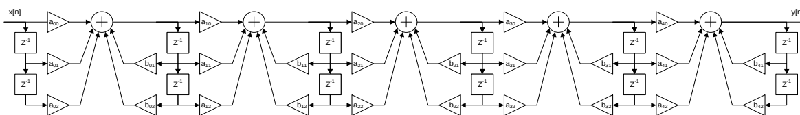
Figure 22. Cascade of five biquad filter stages
