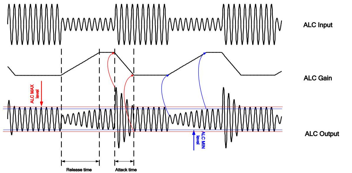
Figure 11. Principle of operation of the ALC
