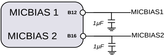
Figure 38. MICBIAS decoupling
