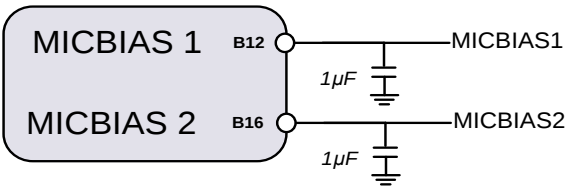
Figure 38. MICBIAS decoupling
