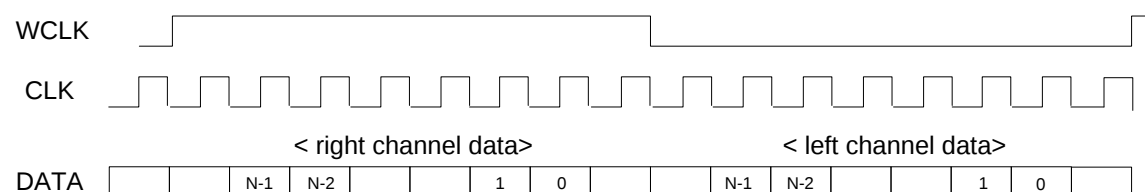
Figure 35: I2S Format
