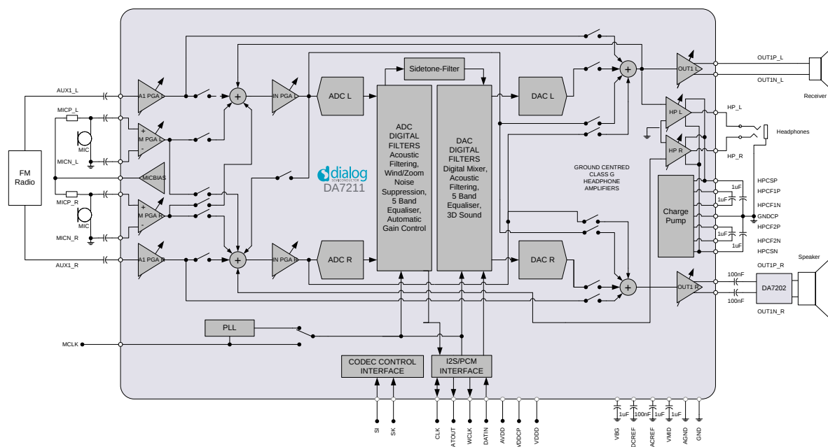
Figure 1: DA7211 Block Diagram
