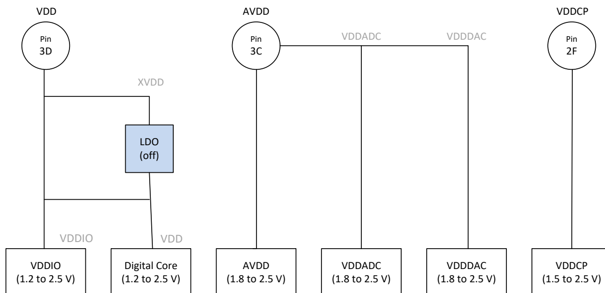
Figure 3: DA7211 Power Supply Topology
