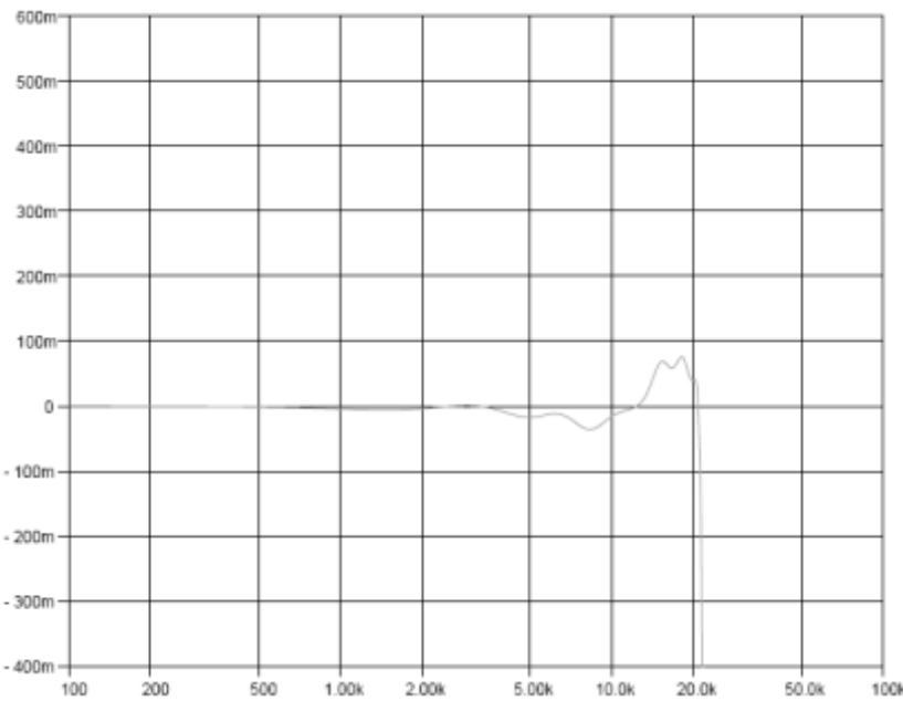
Figure 8: ADC Pass Band Attenuation (Audio Mode, 48 kHz)
