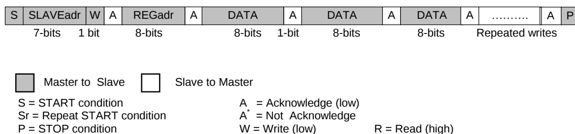
Figure 47: 2-Wire Page Write (SI/DATA Line)
