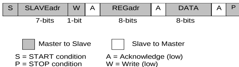
Figure 44: 2-Wire Byte Write (SI/DATA Line)
