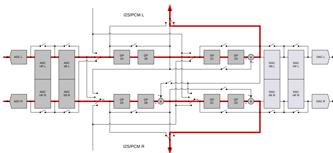
Figure 22: Record Only
