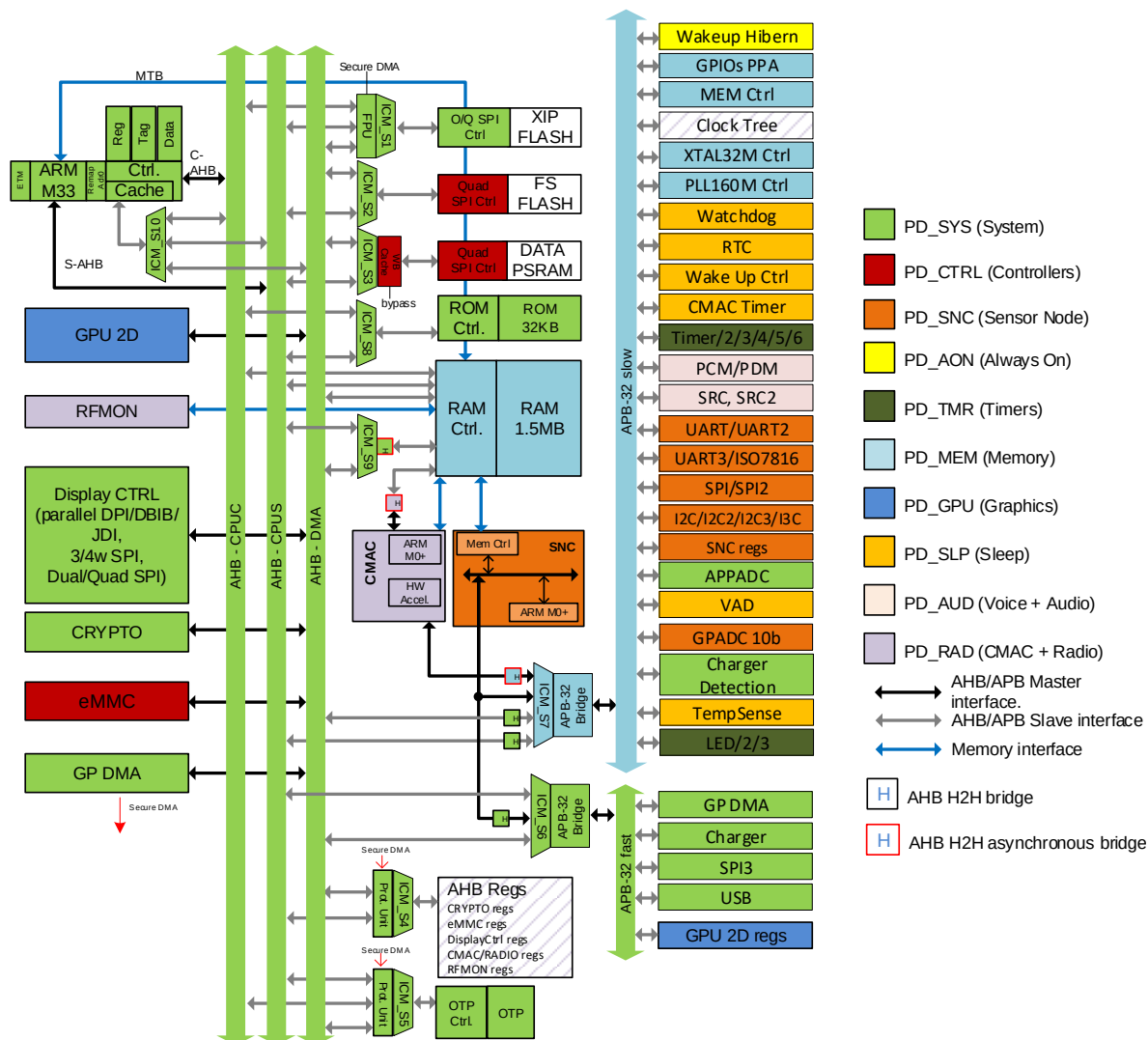
Figure 33: Bus Architecture
