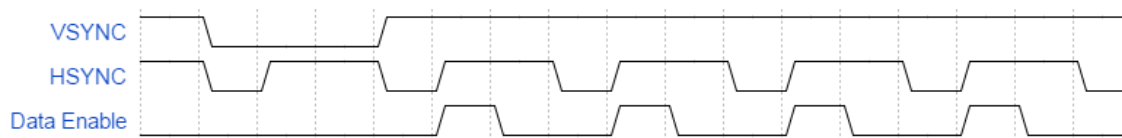
Figure 53: HSYNC/VSNC Typical Waveform
