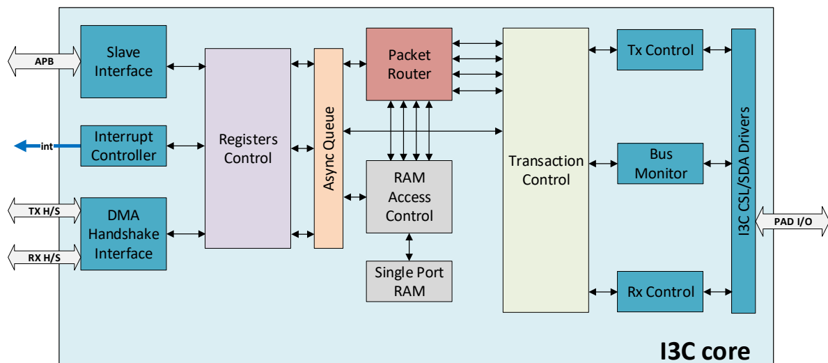
Figure 78: I3C Controller Block Diagram
