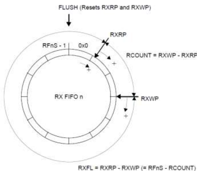
Figure 106: USB Rx FIFO Operation
