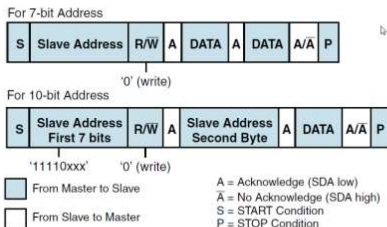
Figure 83: Master-Transmitter Protocol
