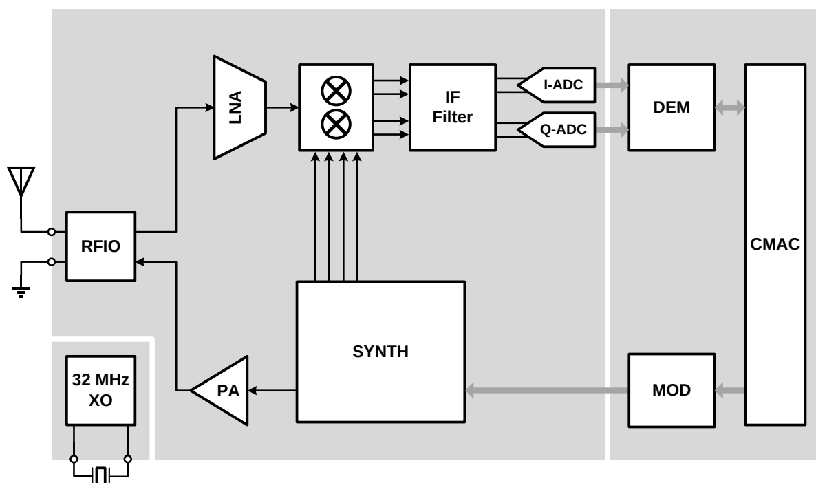
Figure 114: Radio Block Diagram
