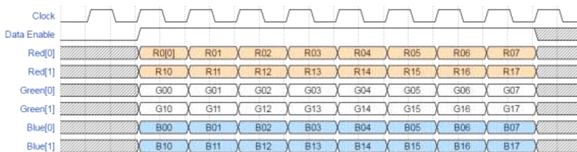
Figure 54: HSYNC/VSNC Color Bits Waveform
