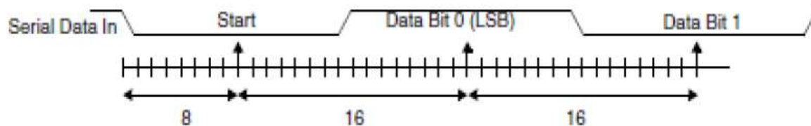
Figure 91: Receiver Serial Data Sampling Points
