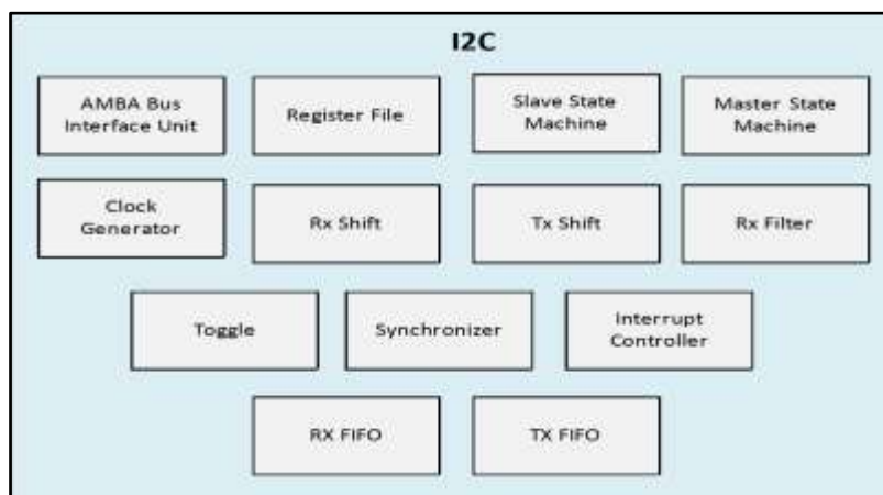
Figure 78: I2C Controller Block Diagram
