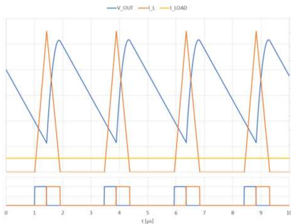
Figure 17: DC-DC Boost Principle
