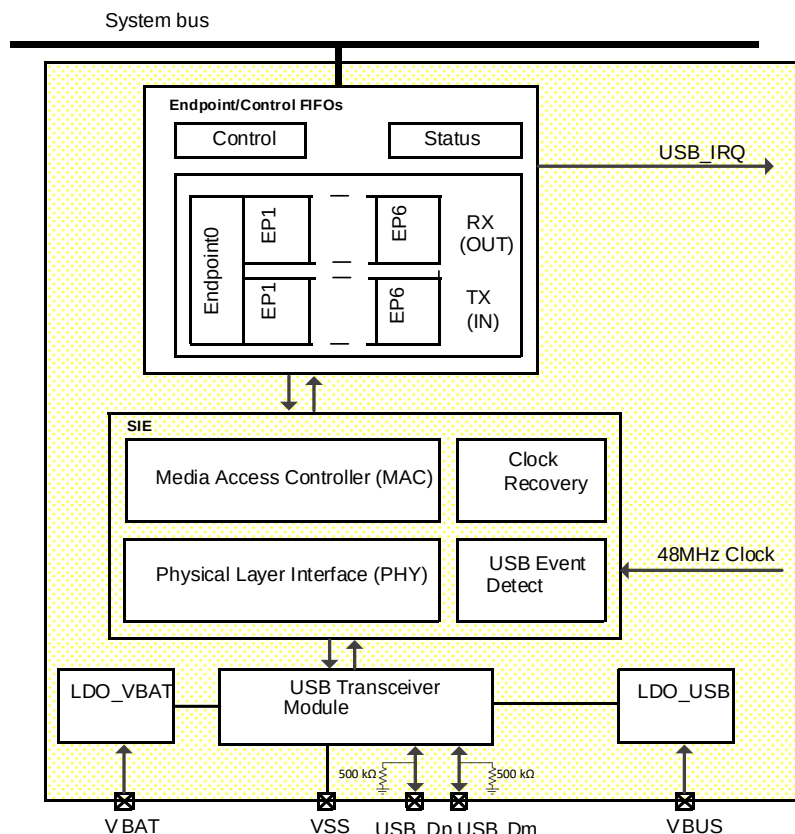
Figure 100: USB Node Block Diagram
