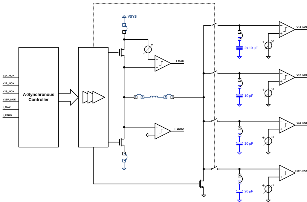
Figure 15: SIMO Buck Converter Block Diagram
