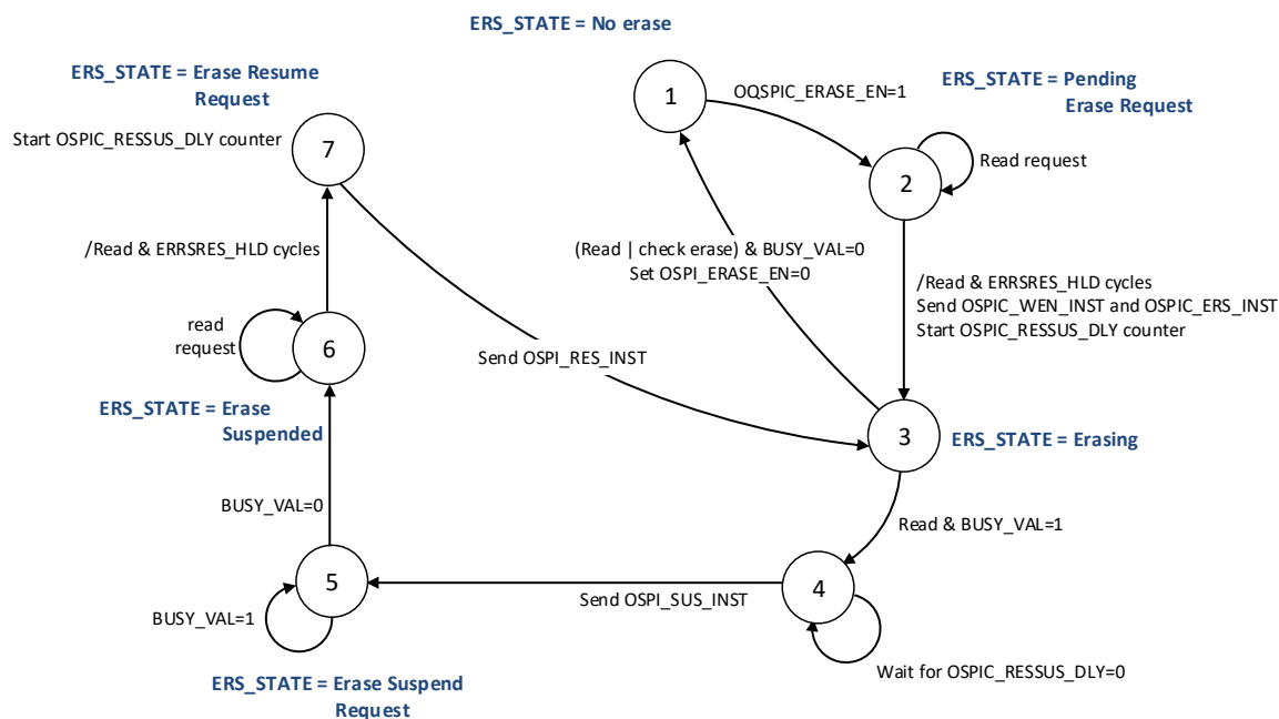
Figure 44: Erase Suspend/Resume in Auto Mode
