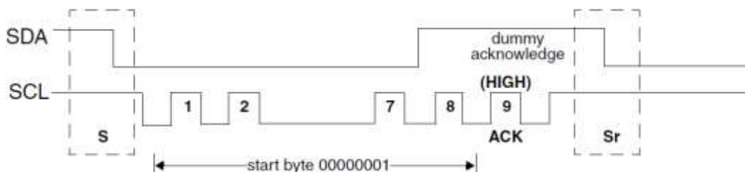
Figure 85: START BYTE Transfer
