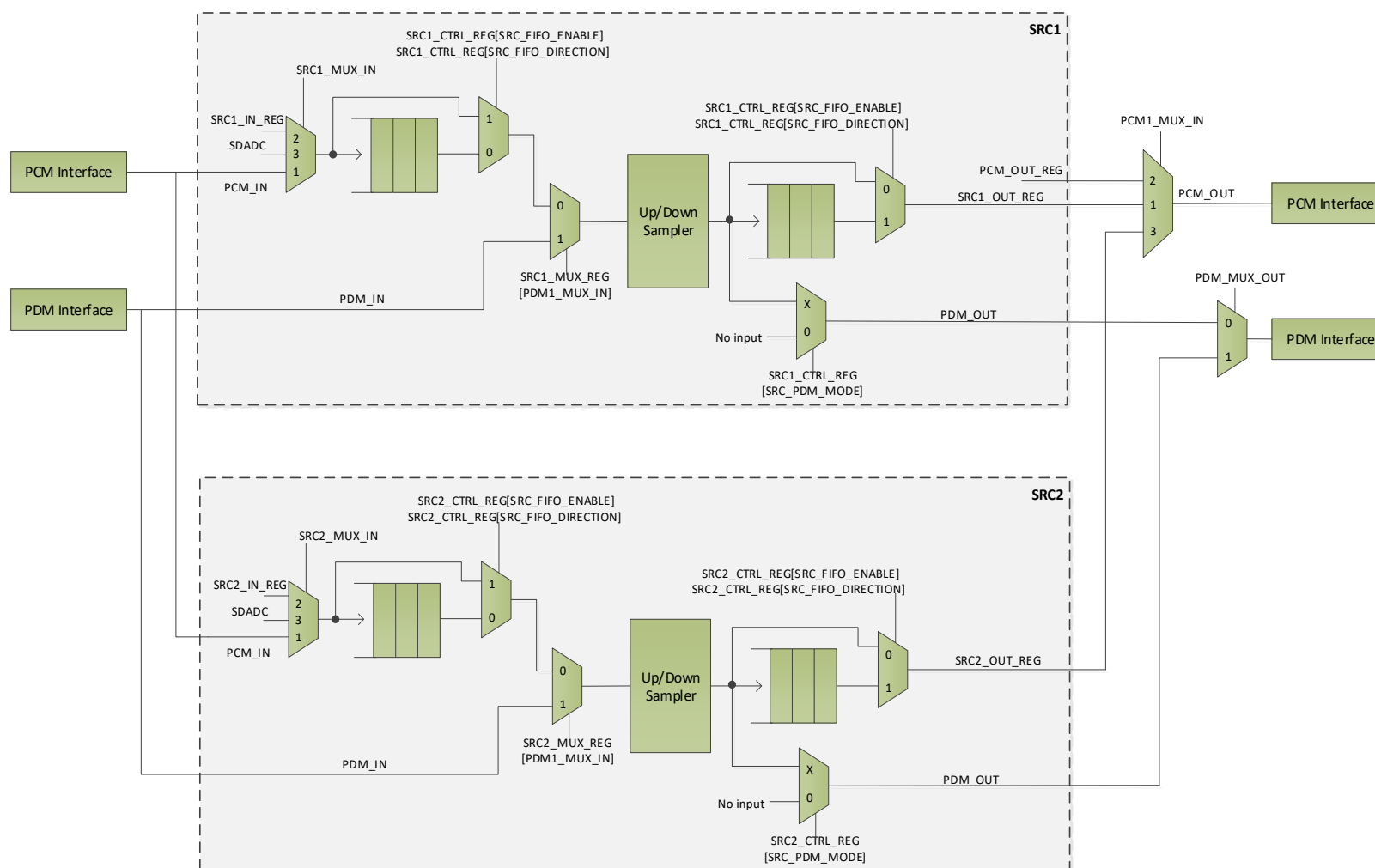
Figure 67: Audio Unit Block Diagram
