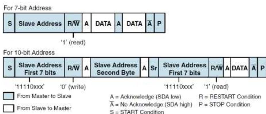
Figure 84: Master-Receiver Protocol
