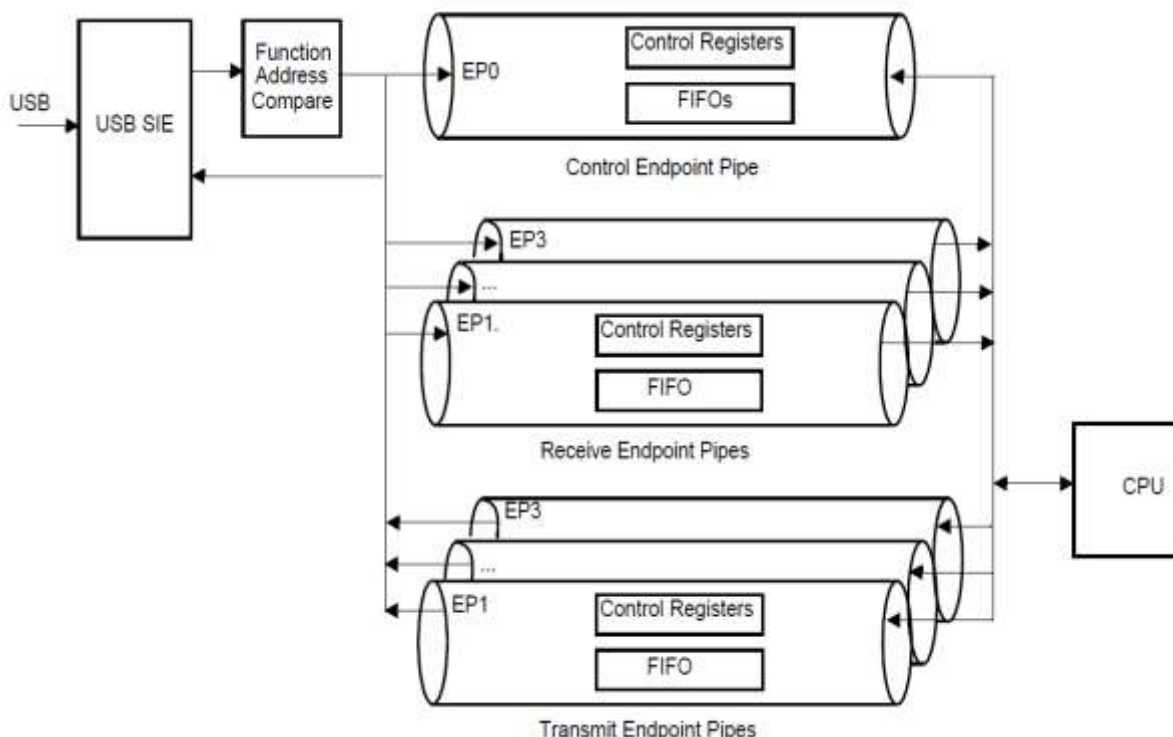
Figure 101: Endpoint Operation
