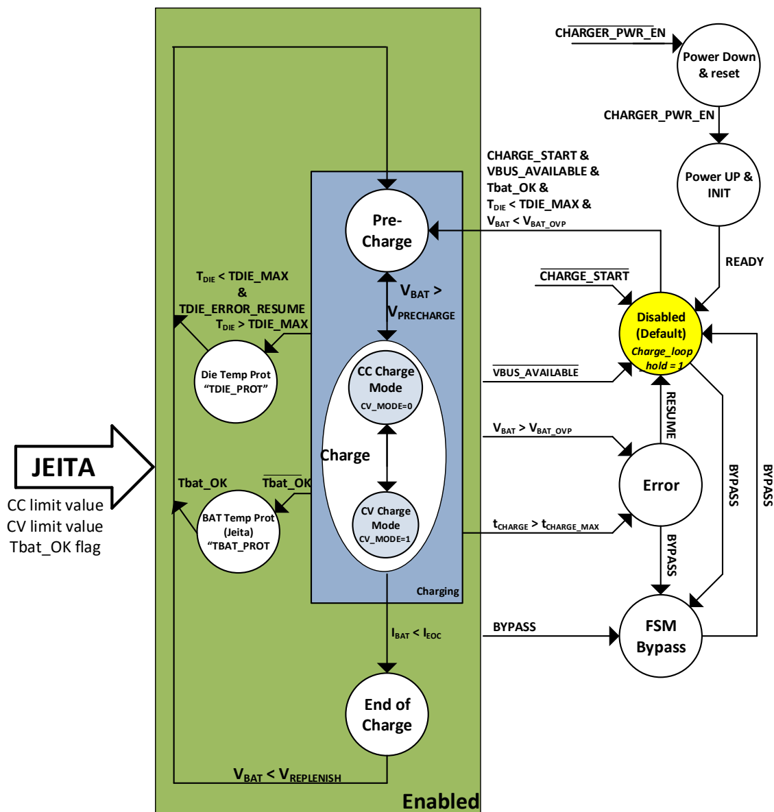
Figure 18: Charger FSM
