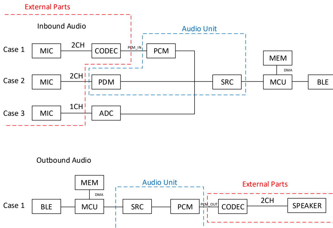
Figure 68: Inbound and Outbound Audio Streams Data Paths
