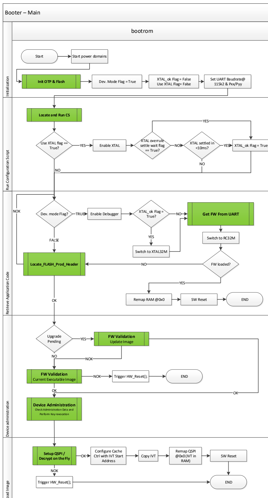
Figure 13: BootROM Flowchart
