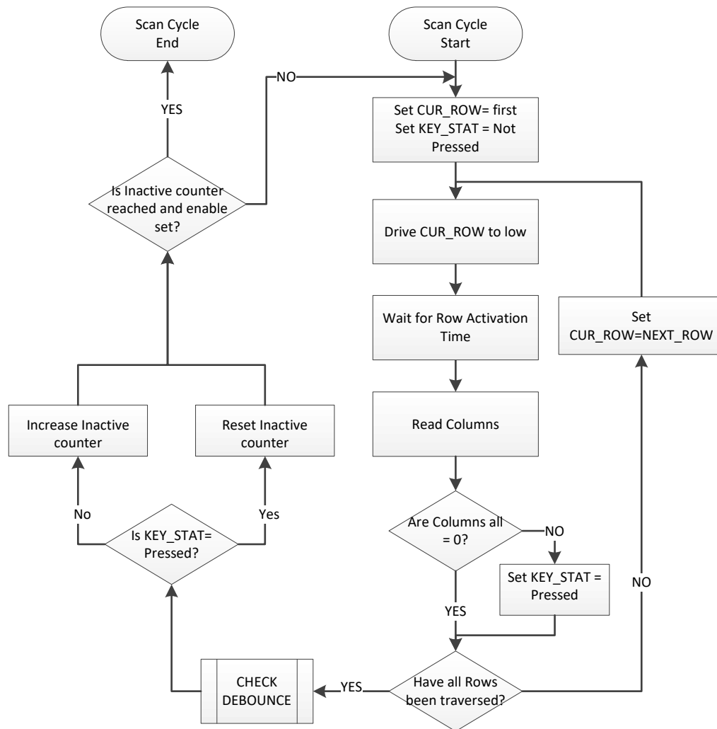
Figure 102: Scan cycle state machine
