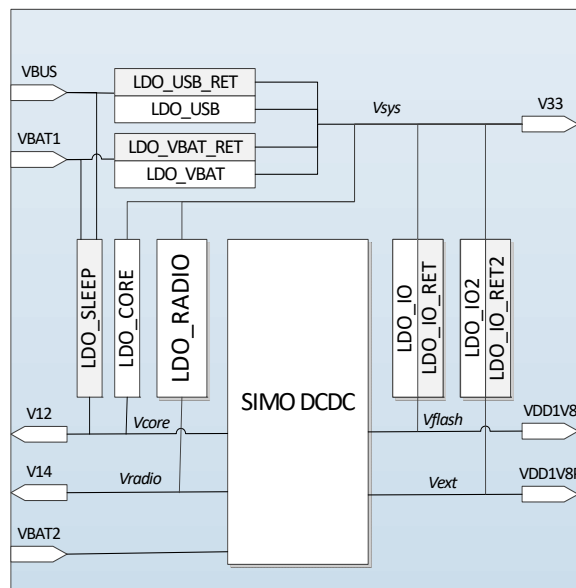
Figure 6: Power Management Unit overview
