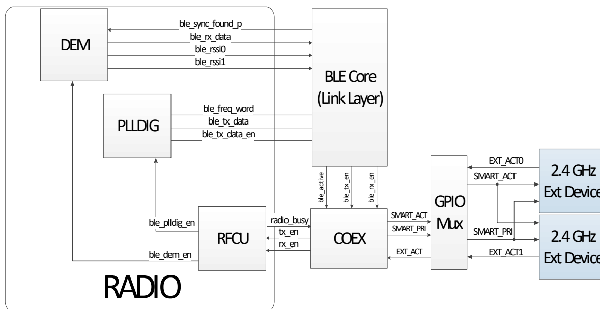
Figure 129: Coexistence interface
