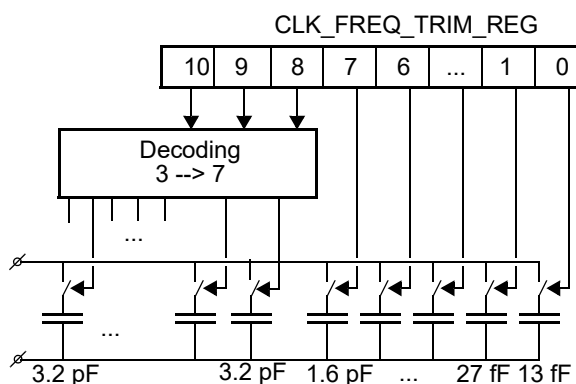
Figure 35: Frequency trimming
