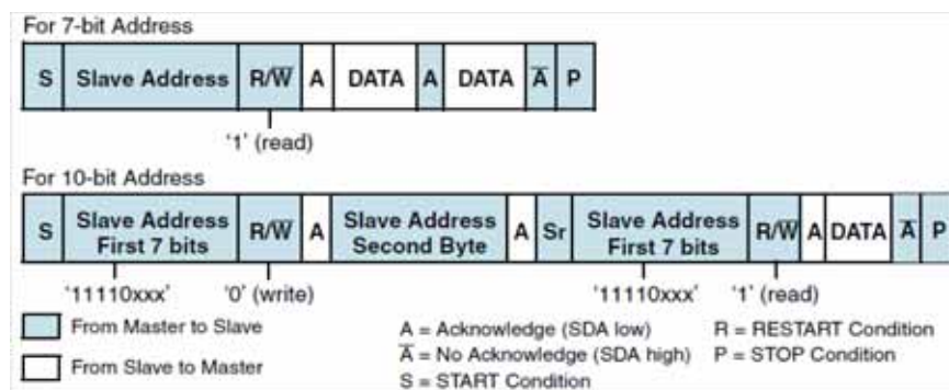
Figure 91: Master-Receiver Protocol
