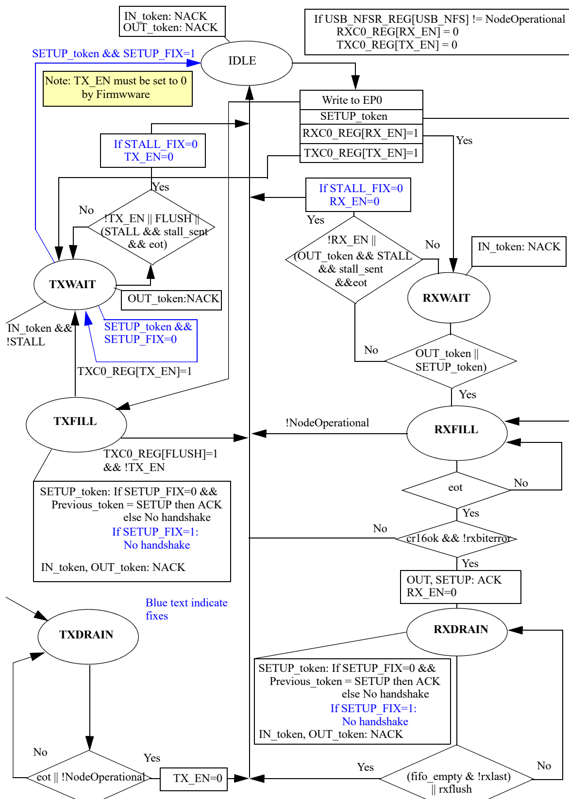
Figure 113: Endpoint 0 Operation
