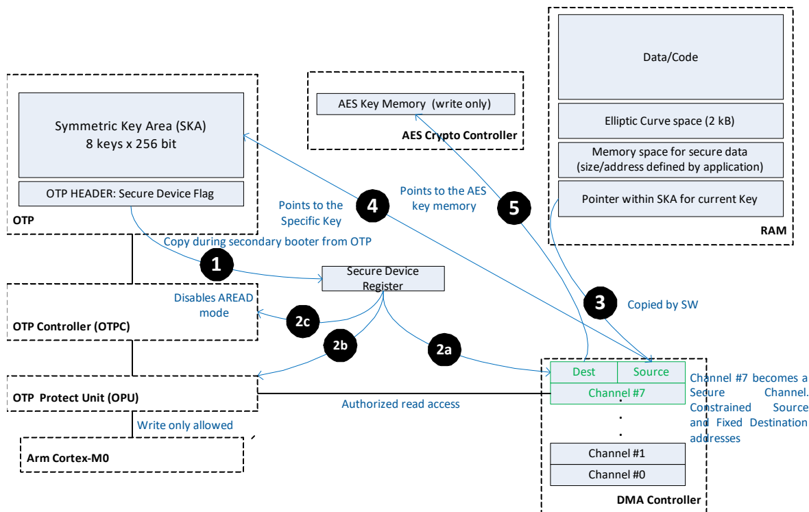
Figure 9: Symmetric Keys manipulation
