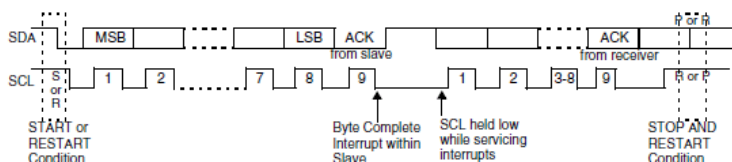
Figure 20: Data Transfer on the I2C Bus
