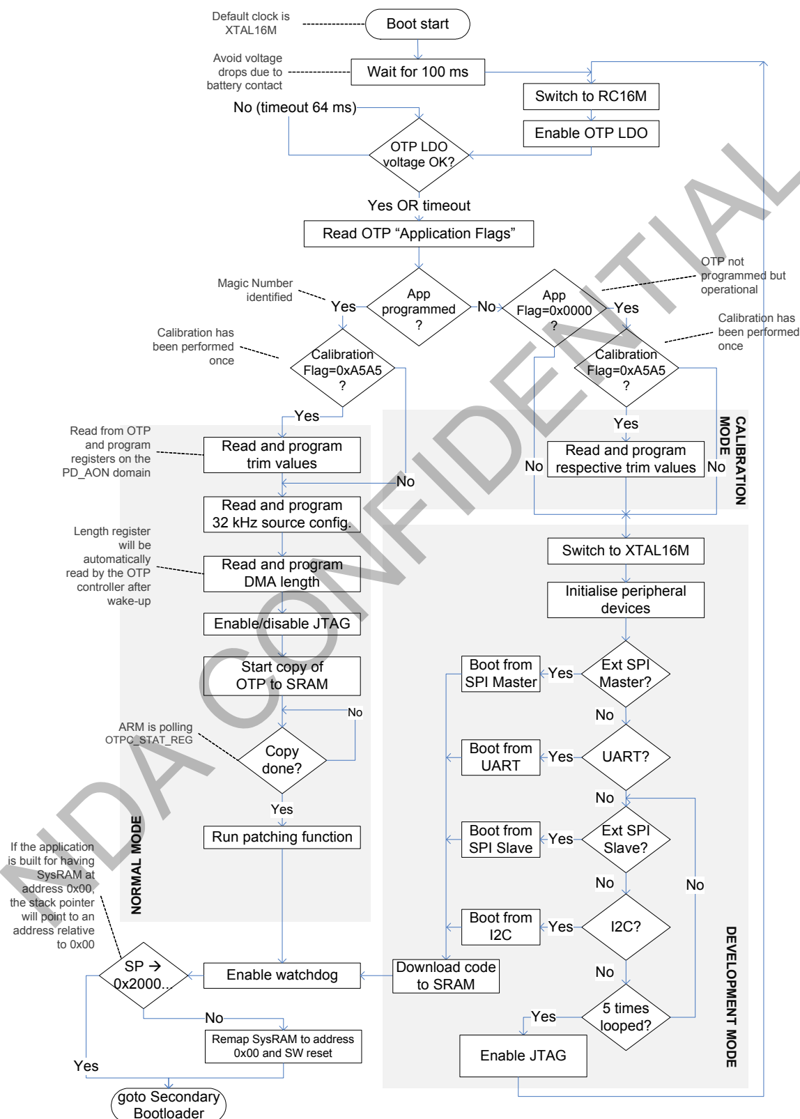
Figure 7: BootROM Sequence
