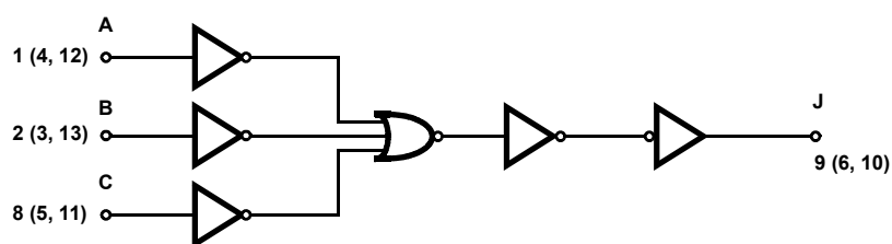
FIGURE 2. LOGIC DIAGRAM FOR CD4073BMS (1 OF 3 IDENTICAL GATES)
