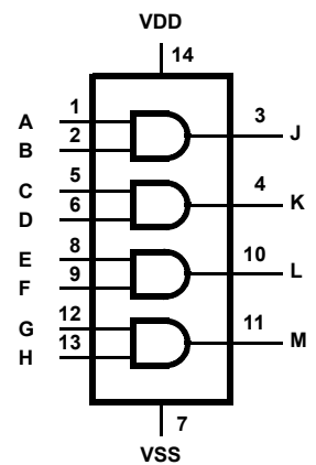
CD4081BMS
