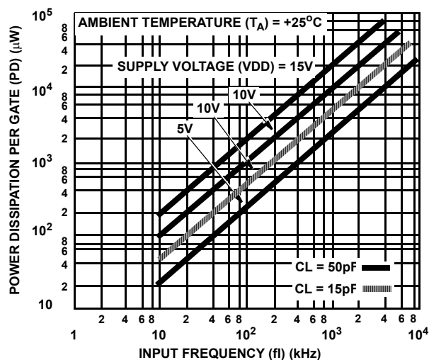
FIGURE 2. TYPICAL POWER DISSIPATION CHARACTERISTICS
