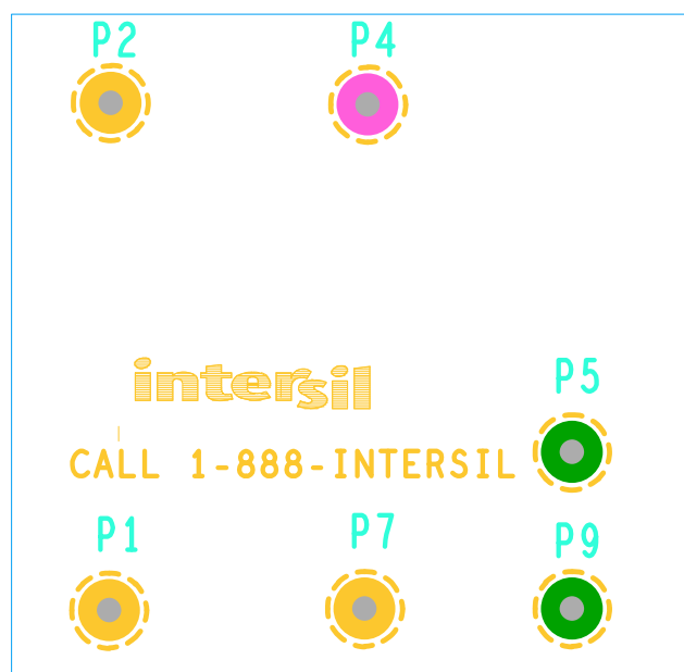
FIGURE 4. SILKSCREEN BOTTOM
