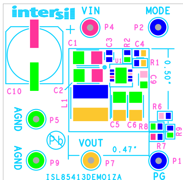
FIGURE 3. SILKSCREEN TOP
