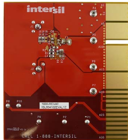
FIGURE 5. BACK OF EVALUATION BOARD ISL854102EVAL1Z
