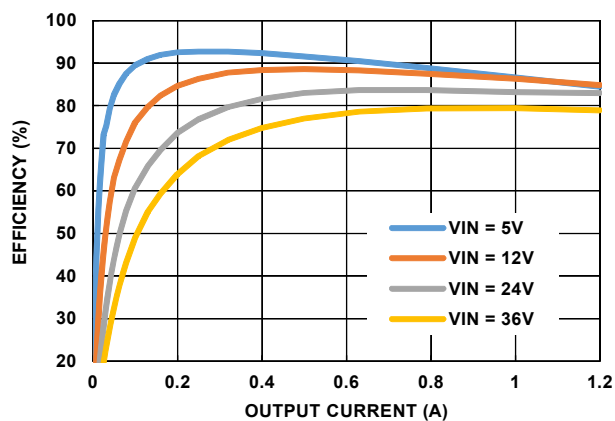
FIGURE 20. EFFICIENCY, PWM (ISL854102EVAL1Z, V_{OUT} = 3.3V )
