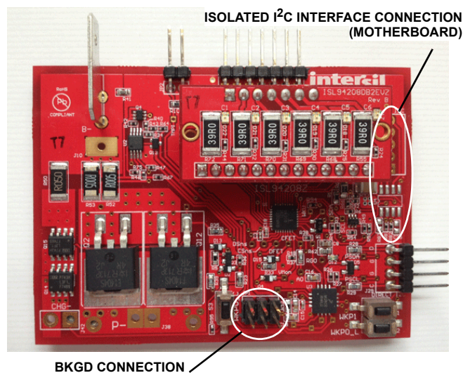
FIGURE 14. ISL94208EVZ ISOLATED INTERFACE AND BKGD CONNECTIONS
