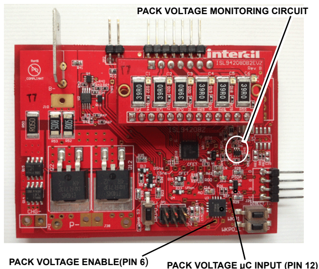
FIGURE 10. ISL94208EVZ PACK VOLTAGE MONITORING CONNECTIONS
