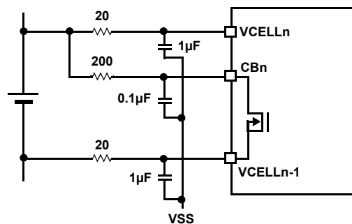
FIGURE 12. ISL94208DB1EVZ VCELL AND CB CONNECTION
