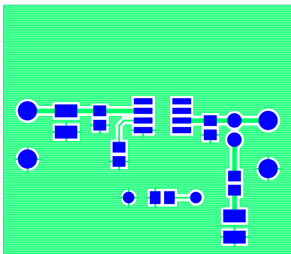
FIGURE 2. TOP COMPONENTS
