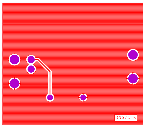
FIGURE 3. BOTTOM LAYER
