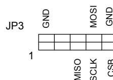
FIGURE 3. JP3 PINOUT
