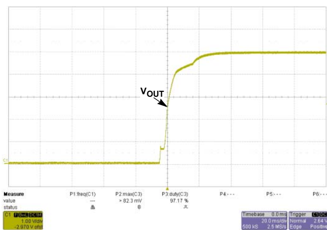
FIGURE 32. RECOVERY @ 33.1V, I_O = 0A
