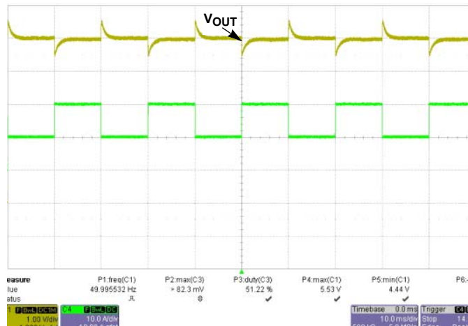
FIGURE 57. \pm 530\text{mV} @ 25%-50%-25% LOAD, 0.2\text{A}/\mu\text{s} , V_{\text{IN}} = 36\text{V} (YELLOW = V_{\text{O}} , GREEN = I_{\text{O}} )
