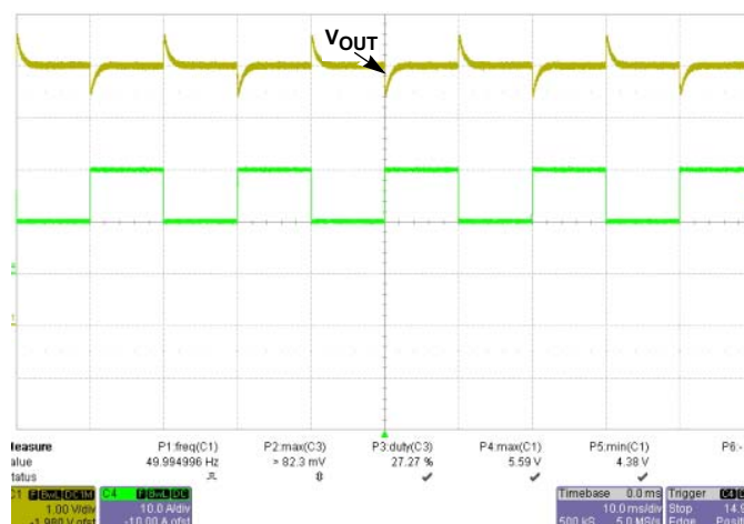
FIGURE 61. \pm 600\text{mV} @ 25%-50%-25% LOAD, 0.2\text{A}/\mu\text{s} , V_{\text{IN}} = 75\text{V} (YELLOW = V_{\text{O}} , GREEN = I_{\text{O}} )
