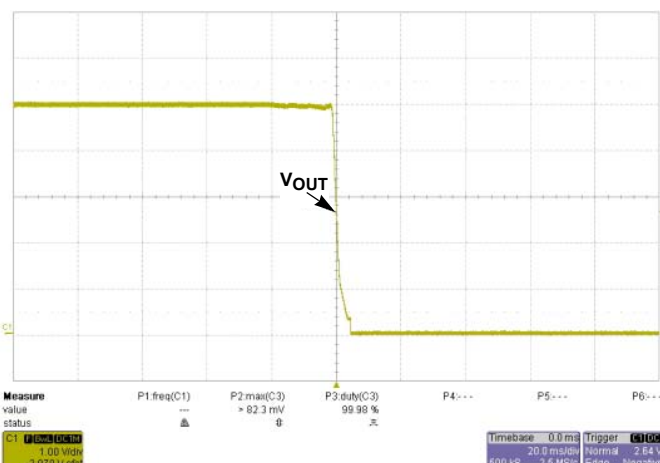
FIGURE 26. SHUT-DOWN AT V_{IN} = 48V @ I_O = 40A
