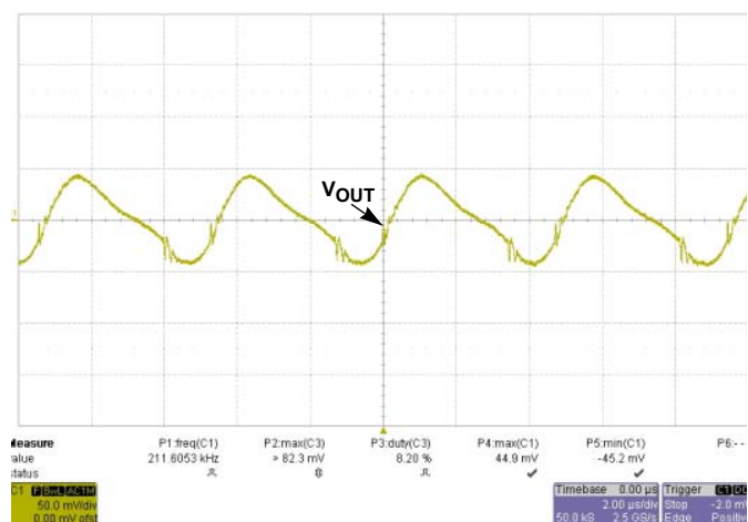
FIGURE 55. PEAK-TO-PEAK = 93mV @ V_{IN} = 75V , I_O = 40A
