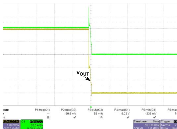
FIGURE 46. I_O OVERSHOOT, SHORT @ V_{IN} = 48V , I_O = 40A
