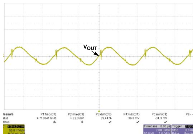
FIGURE 53. PEAK-TO-PEAK = 77mV @ V_{IN} = 48V , I_O = 40A
