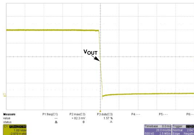
FIGURE 20. SHUT-DOWN AT V_{IN} = 36V @ I_O = 0A
