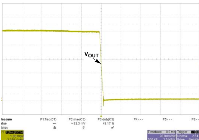
FIGURE 16. SHUT-DOWN AT V_{IN} = 75V @ I_O = 0A
