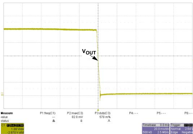
FIGURE 12. SHUT-DOWN AT V_{IN} = 48V @ I_O = 0A
