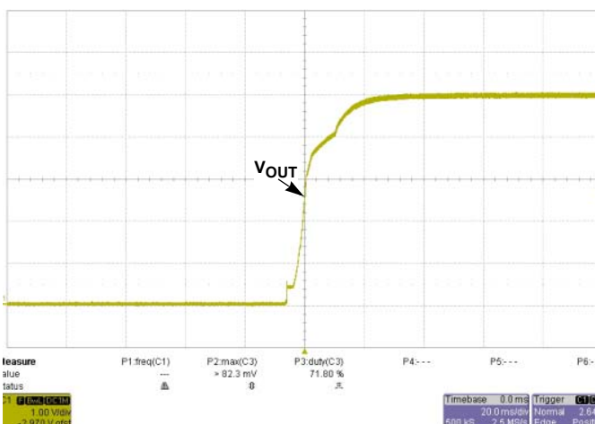
FIGURE 34. RECOVERY @ 33V, I_O = 40A
