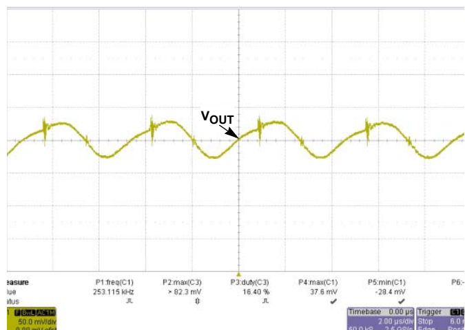
FIGURE 51. PEAK-TO-PEAK = 66mV @ V_{IN} = 36V , I_O = 40A
