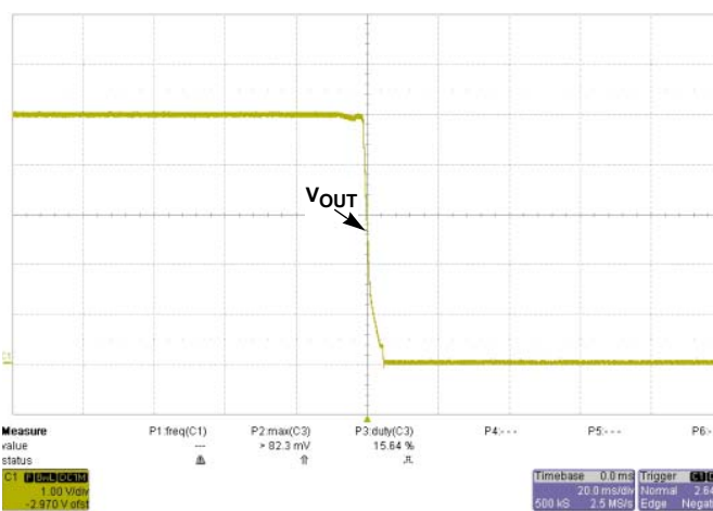
FIGURE 10. SHUT-DOWN AT V_{IN} = 36V @ I_O = 40A
