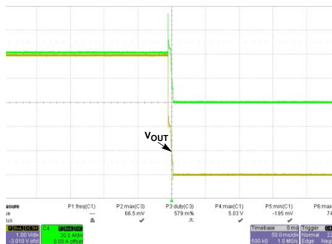
FIGURE 45. I_O OVERSHOOT, SHORT @ V_{IN} = 36V , I_O = 40A
