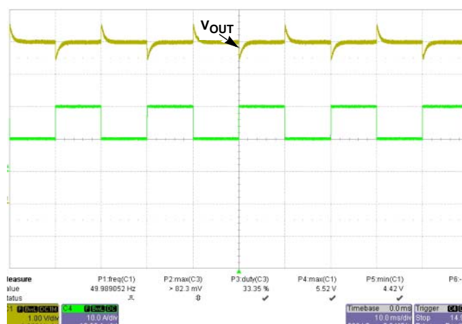
FIGURE 59. \pm 540\text{mV} @ 25%-50%-25% LOAD, 0.2\text{A}/\mu\text{s} , V_{\text{IN}} = 48\text{V} (YELLOW = V_{\text{O}} , GREEN = I_{\text{O}} )
