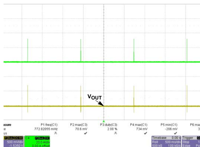
FIGURE 48. START-UP @ OUTPUT TERMINAL SHORT, V_{IN} = 48V
