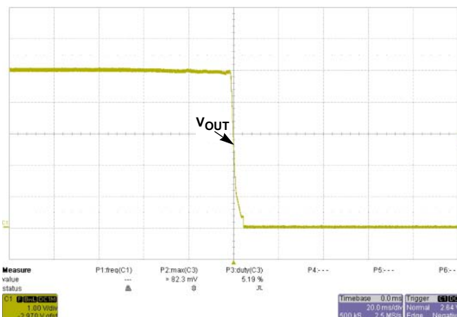
FIGURE 30. SHUT-DOWN AT V_{IN} = 75V @ I_O = 40A
