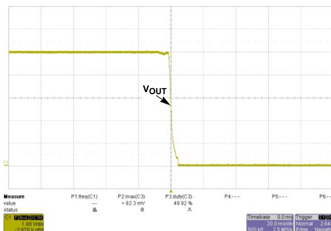
FIGURE 22. SHUT-DOWN AT V_{IN} = 36V @ I_O = 40A
