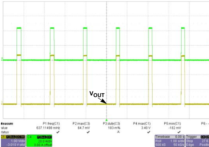
FIGURE 42. OCP = 44.6A @ V_{IN} = 48V (LOAD MODE = CR; YELLOW = V_O , GREEN = I_O )
