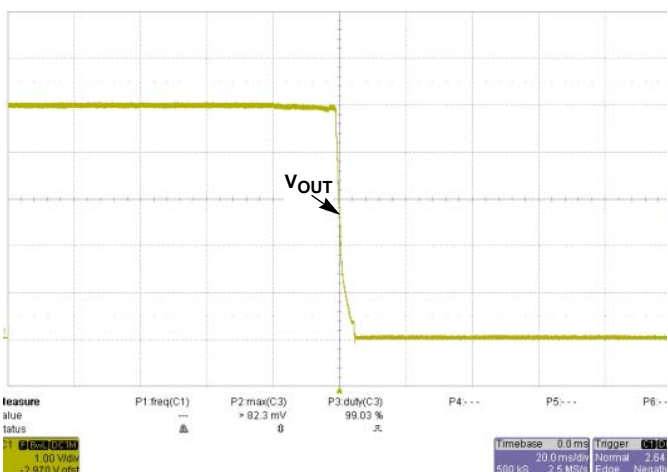
FIGURE 14. SHUT-DOWN AT V_{IN} = 48V @ I_O = 40A
