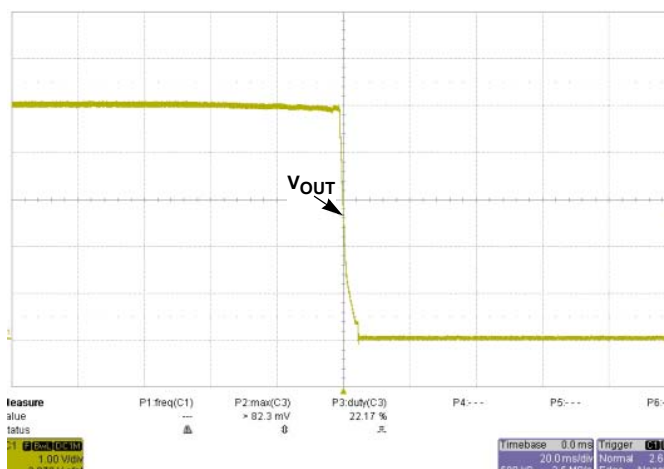
FIGURE 18. SHUT-DOWN AT V_{IN} = 75V @ I_O = 40A
