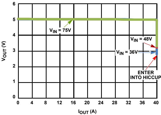
FIGURE 44. OCP CHARACTERISTICS
