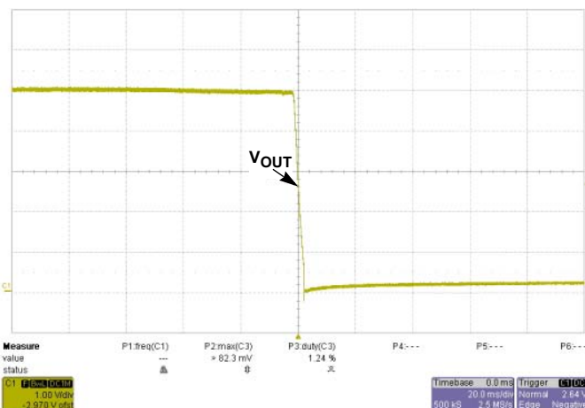
FIGURE 24. SHUT-DOWN AT V_{IN} = 48V @ I_O = 0A
