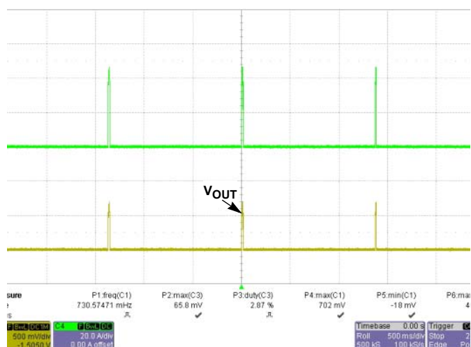
FIGURE 49. START-UP @ OUTPUT TERMINAL SHORT, V_{IN} = 75V
