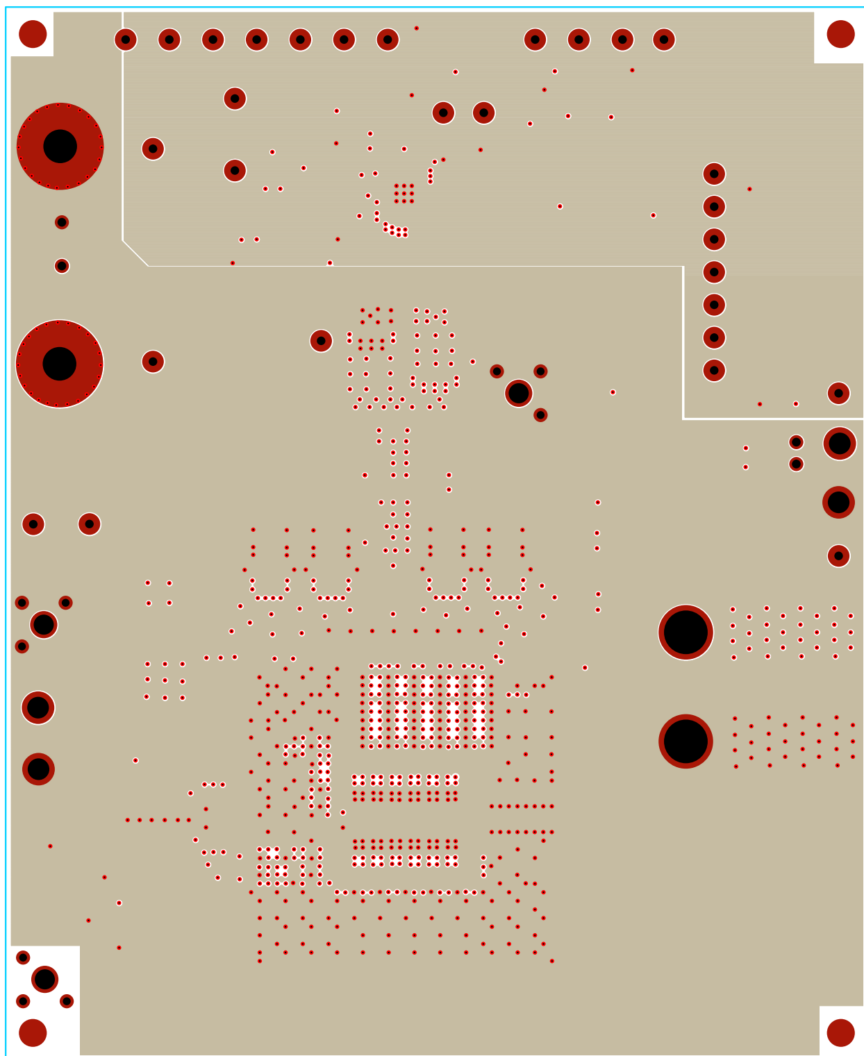
FIGURE 14. LAYER 6
