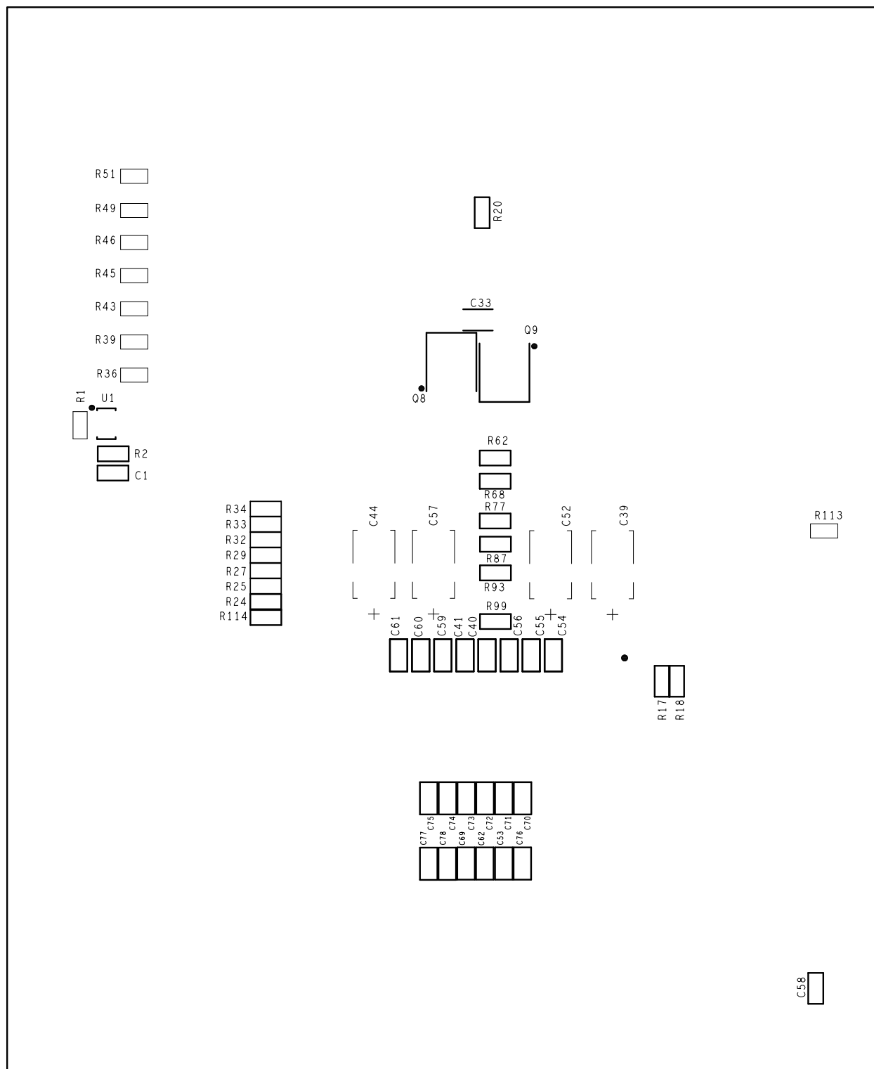
FIGURE 8. BOTTOM SILKSCREEN
