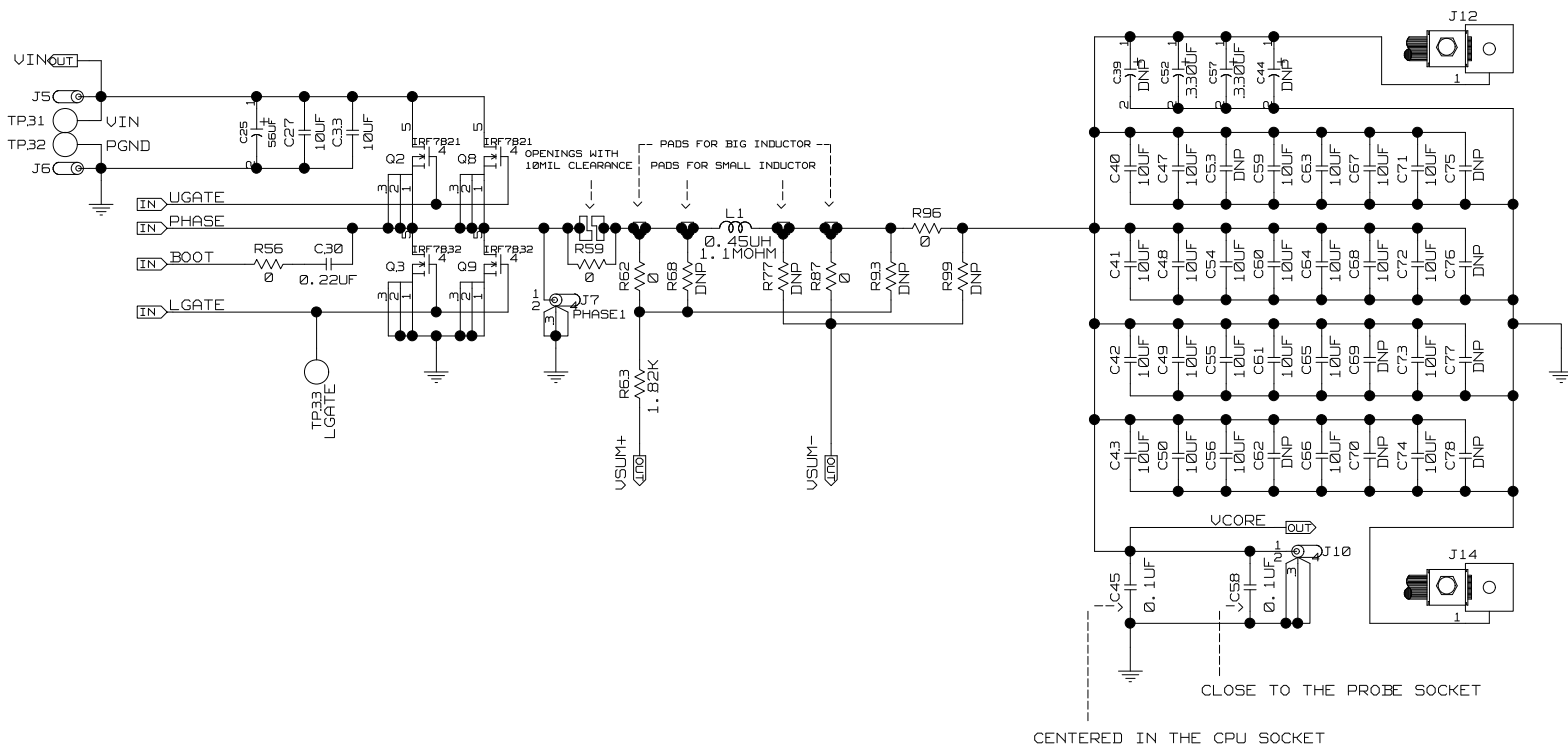
FIGURE 3. ISL62881CCPUEVAL2Z SCHEMATIC, 2 OF 5
