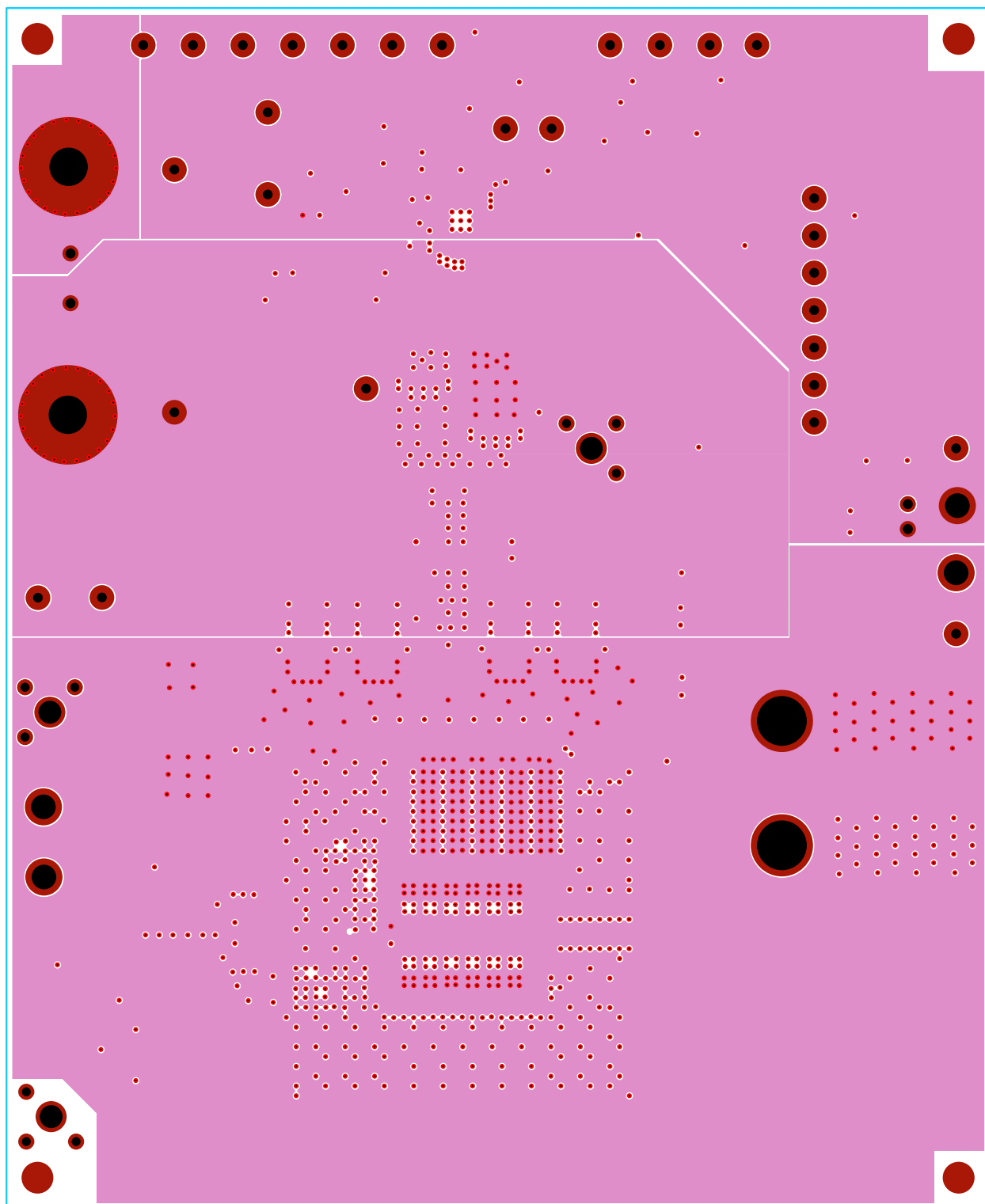
FIGURE 15. LAYER 7
