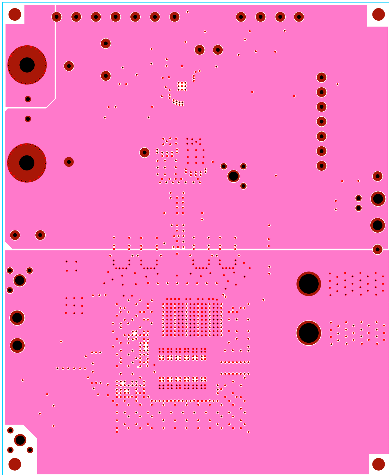
FIGURE 13. LAYER 5
