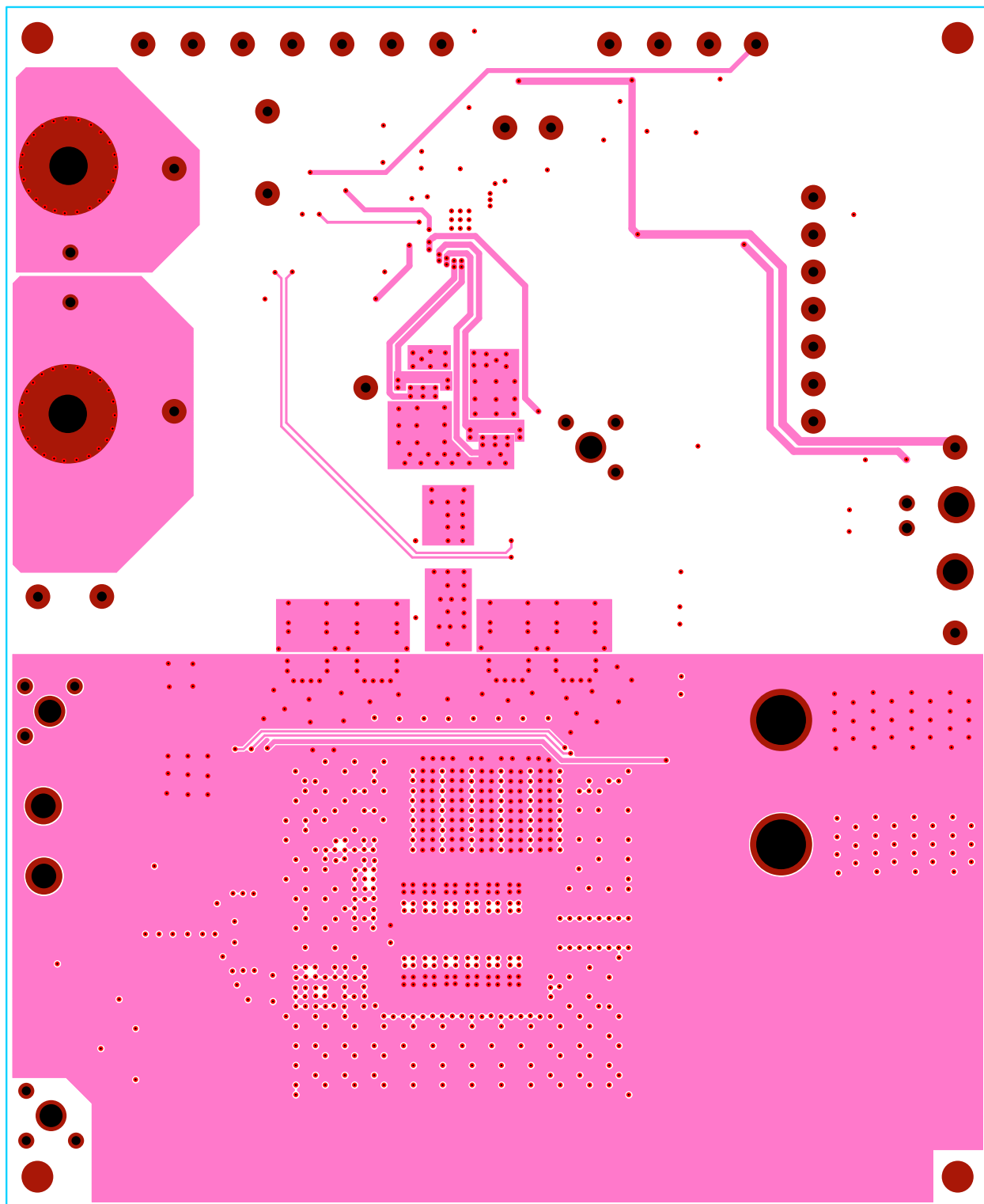
FIGURE 11. LAYER 3
