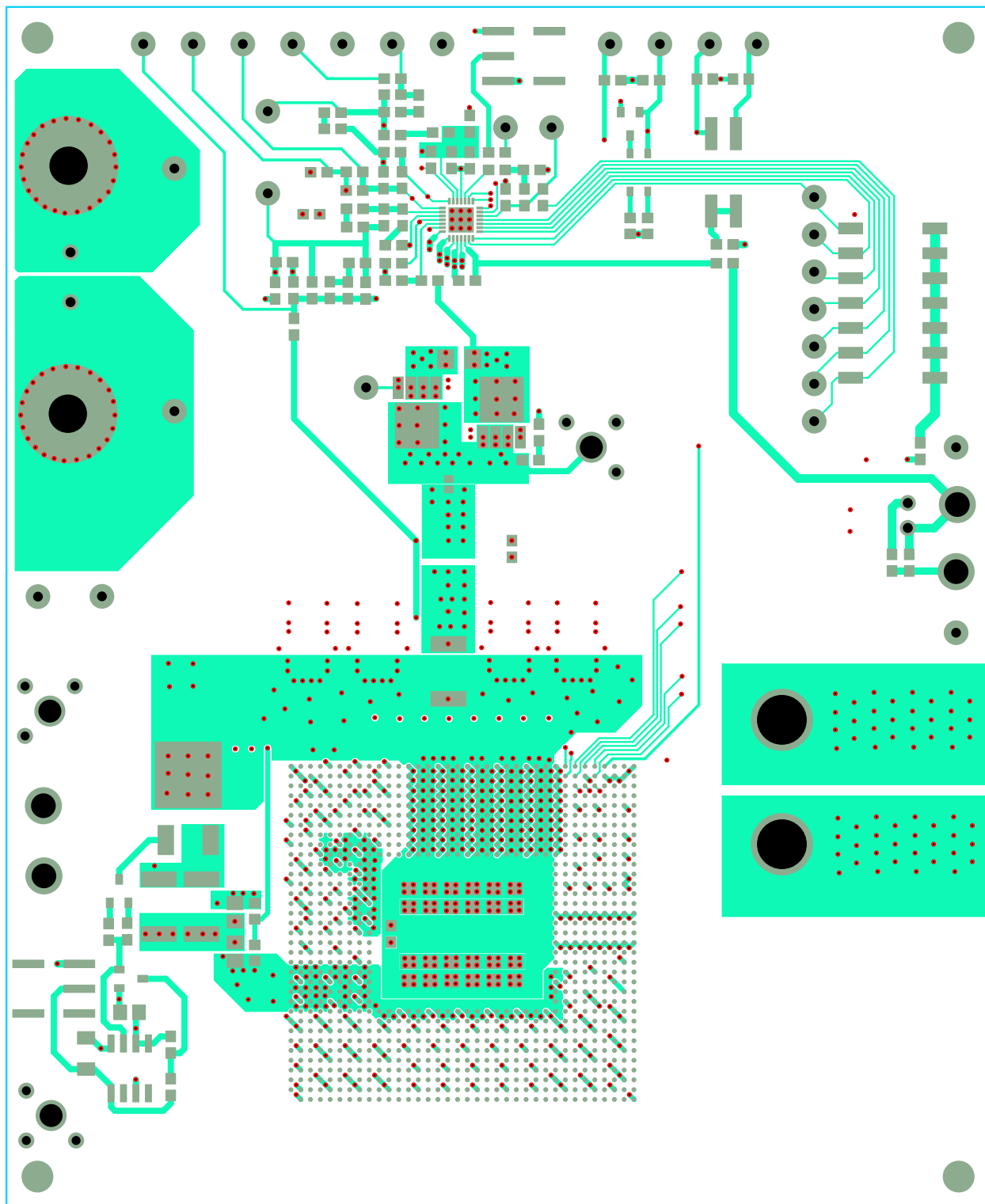
FIGURE 9. LAYER 1
