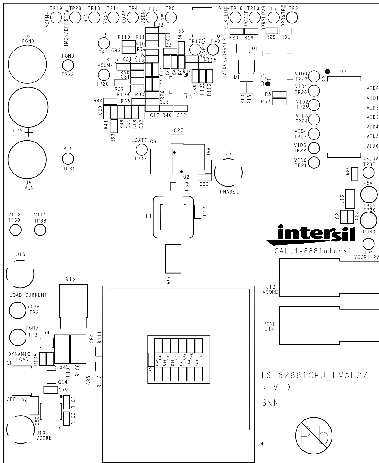
FIGURE 7. TOP SILKSREEN
