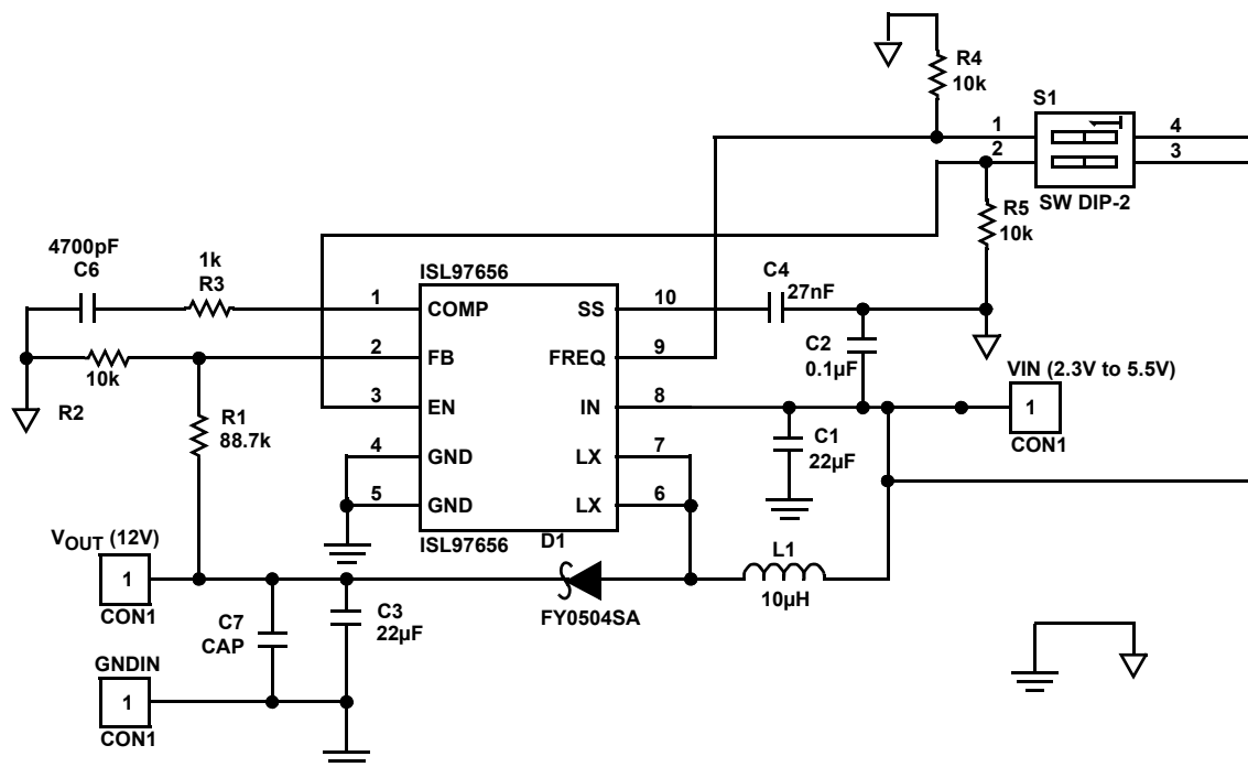
FIGURE 1. SCHEMATIC
