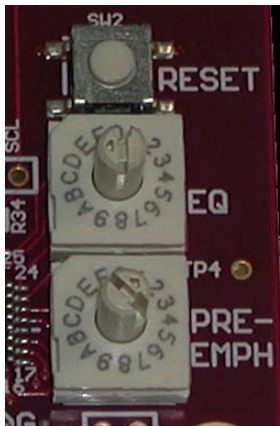
FIGURE 13. ISL54105A ROTARY SWITCHES AND RESET BUTTON
