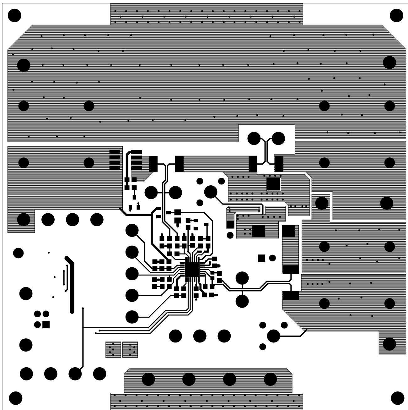
FIGURE 13. TOP COPPER
