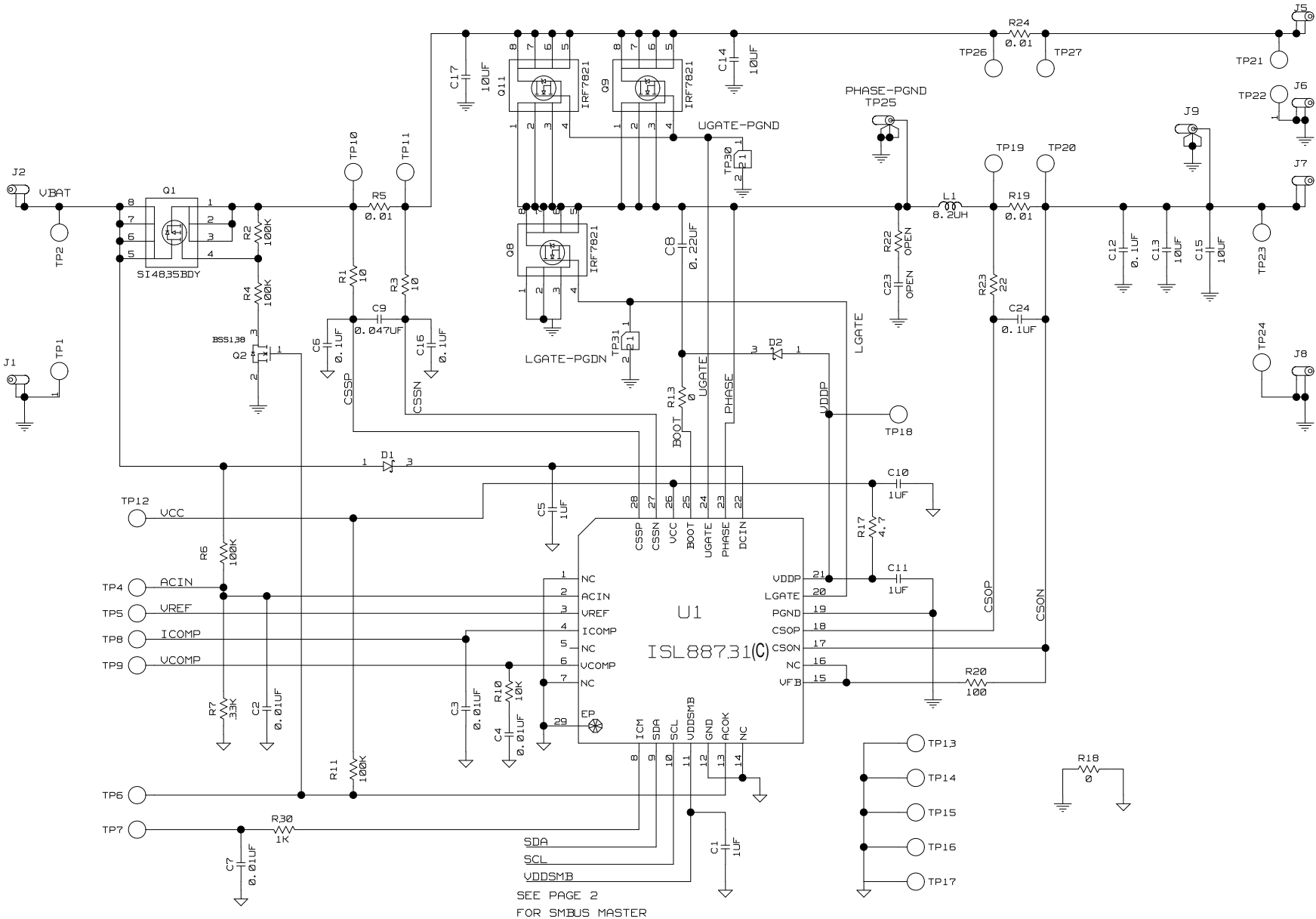
FIGURE 10. ISL88731(C)EVAL2Z SCHEMATIC
