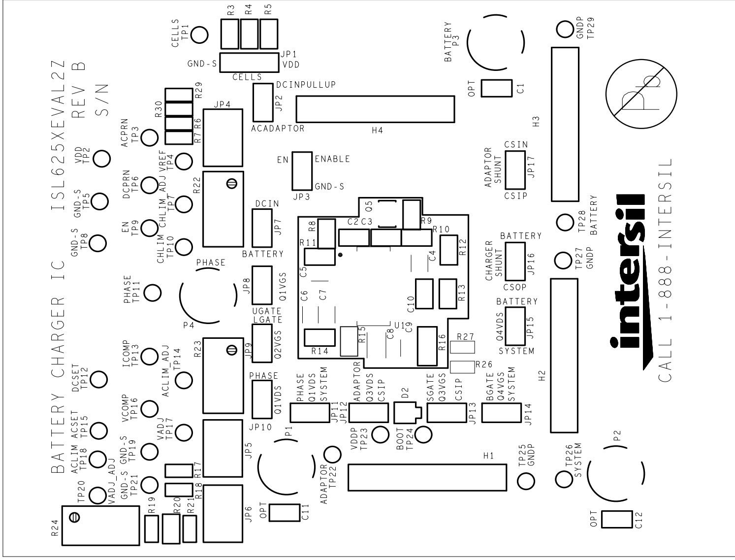
FIGURE 1. TOP SILK
