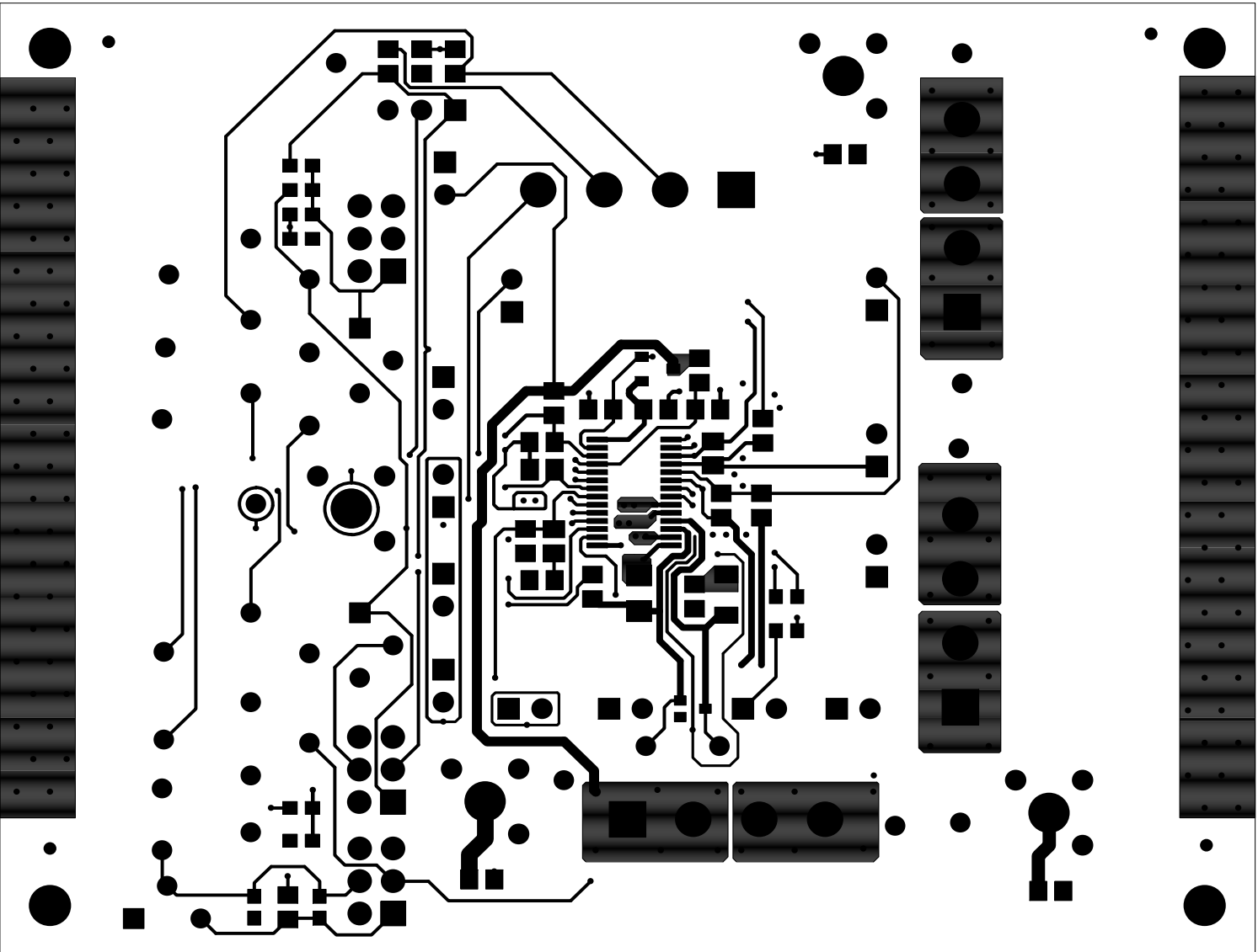
FIGURE 2. TOP LAYER
