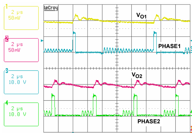
FIGURE 5. DCM STEADY-STATE OPERATION, V_{IN} = 12V , V_{O1} = 1.5V , I_{O1} = 2A , V_{O2} = 1.8V , I_{O2} = 2A
