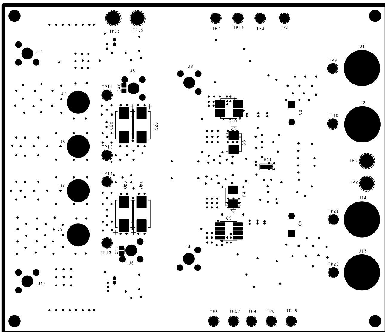
FIGURE 14. BOTTOM SILKSCREEN
