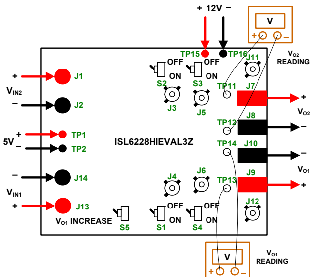
FIGURE 1. TEST SET-UP
