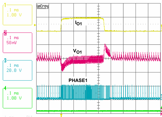
FIGURE 6. TRANSIENT RESPONSE, V_{IN} = 19V , V_O = 1.05V , I_O = 1A/21A @ 2.55A/\mu s
