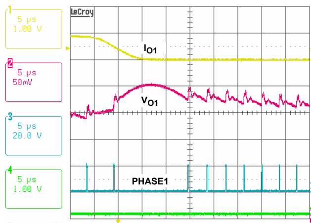
FIGURE 10. LOAD RELEASE RESPONSE, V_{IN} = 19V , V_O = 1.05V , I_O = 1A/21A @ 2.55A/\mu s
