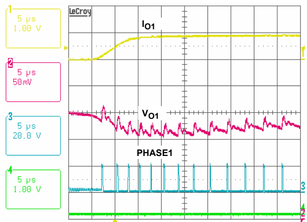
FIGURE 8. LOAD INSERTION RESPONSE, V_{IN} = 19V , V_O = 1.05V , I_O = 1A/21A @ 2.55A/\mu s
