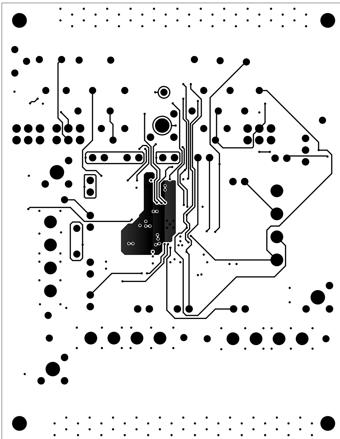
FIGURE 4. LAYER 3 SIGNAL
