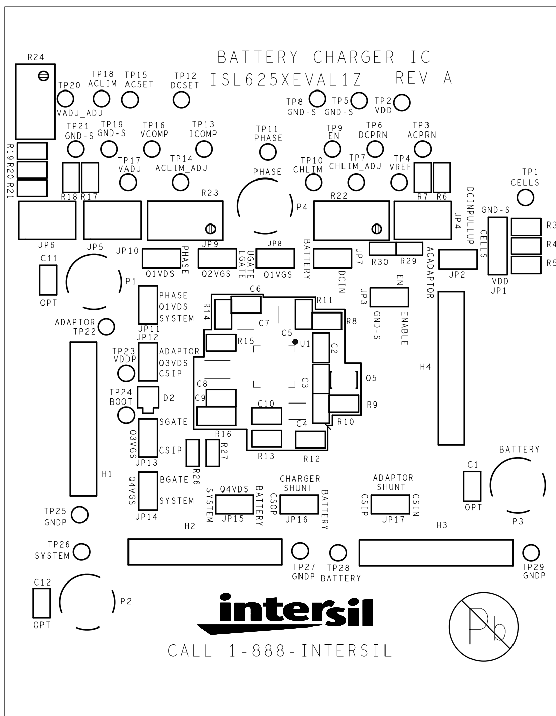
FIGURE 1. TOP SILK
