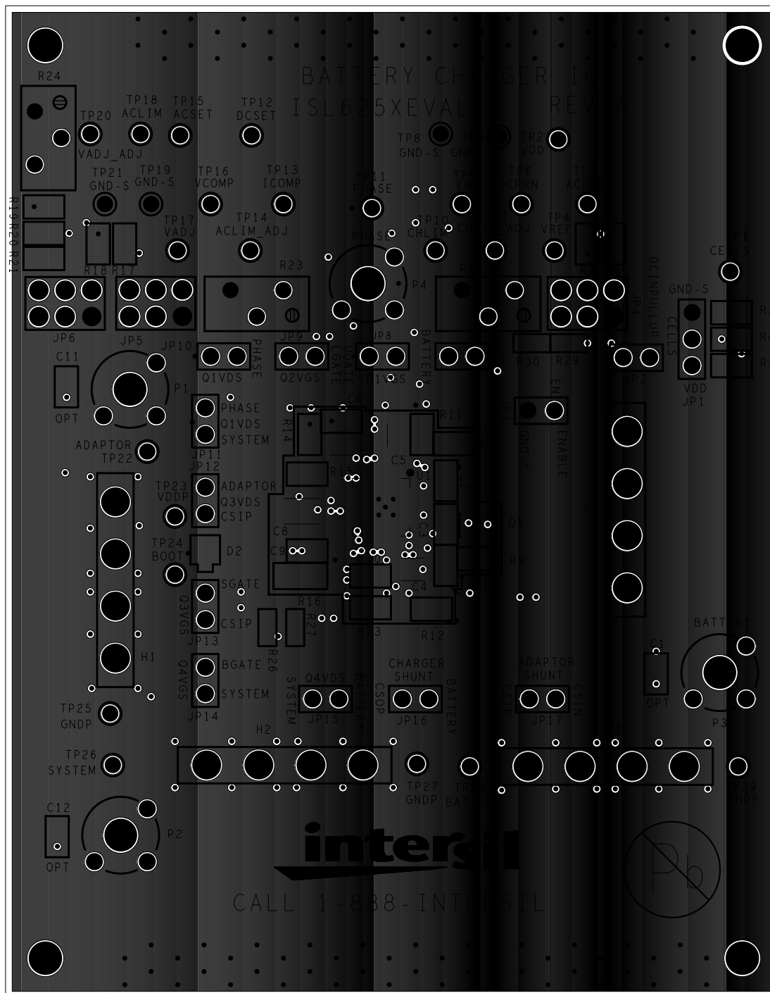
FIGURE 3. LAYER 2 GROUND
