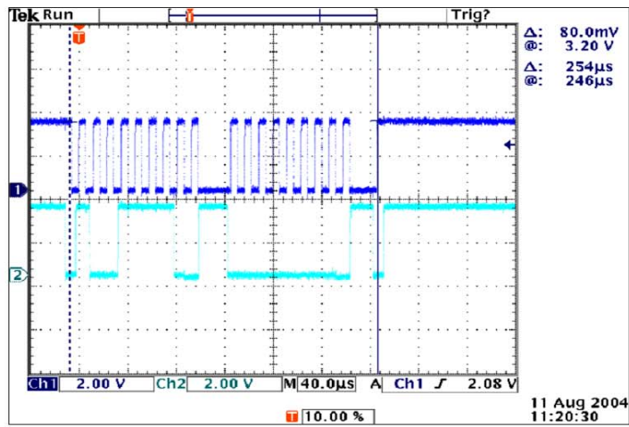
FIGURE 8. ISL45041EVAL1Z TIMING DIAGRAM
