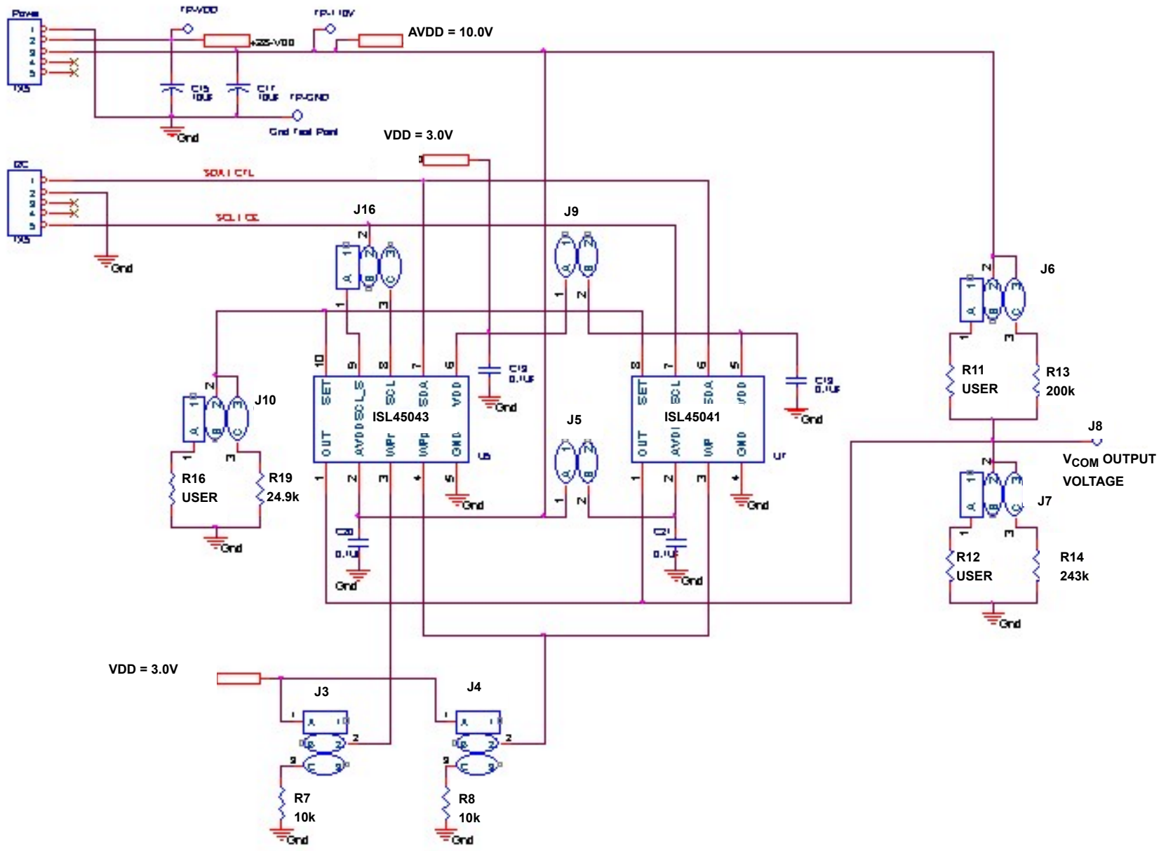
FIGURE 7. ISL45041EVAL1Z SCHEMATIC
