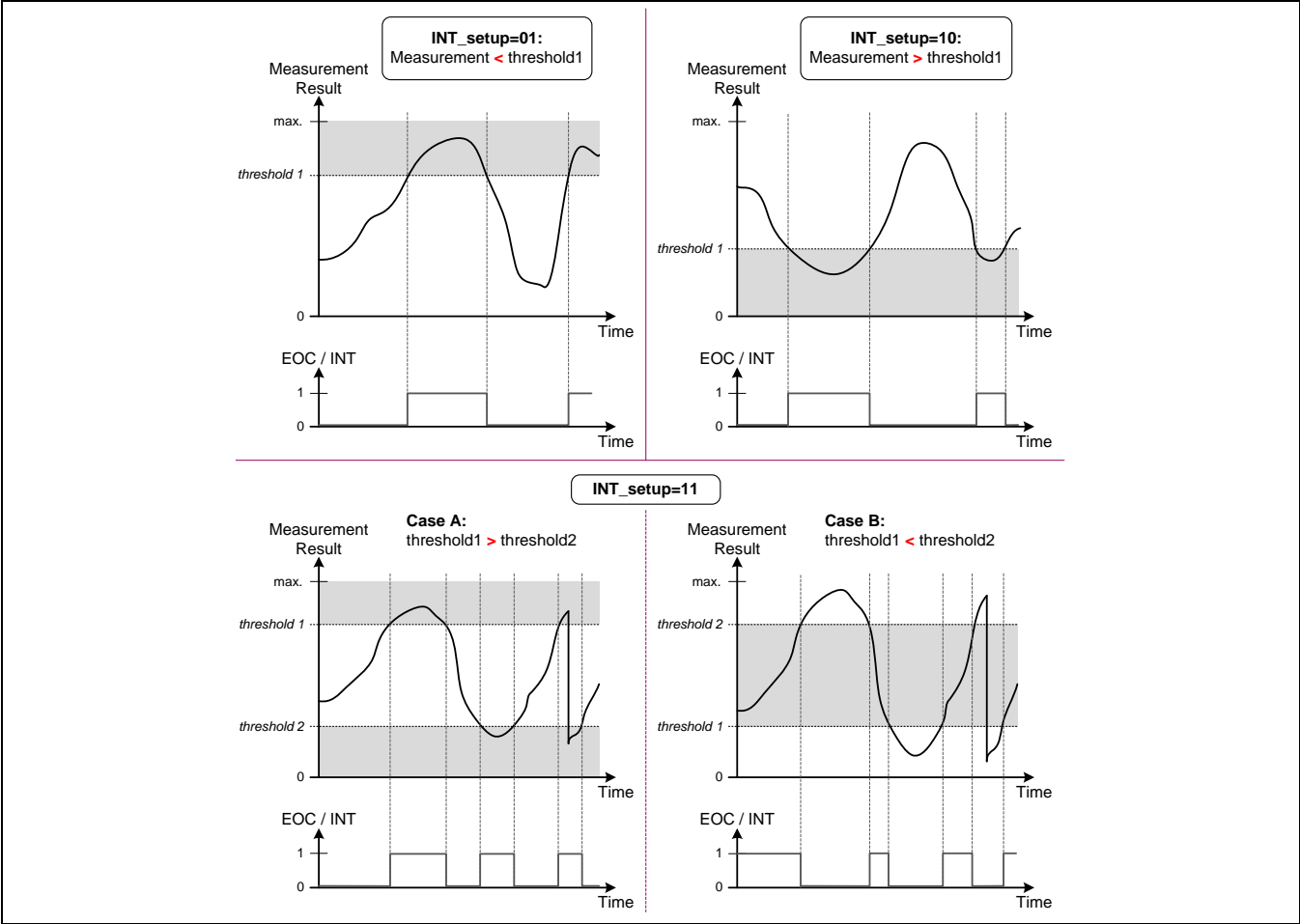
Figure 3.1 Interrupt Functionality
