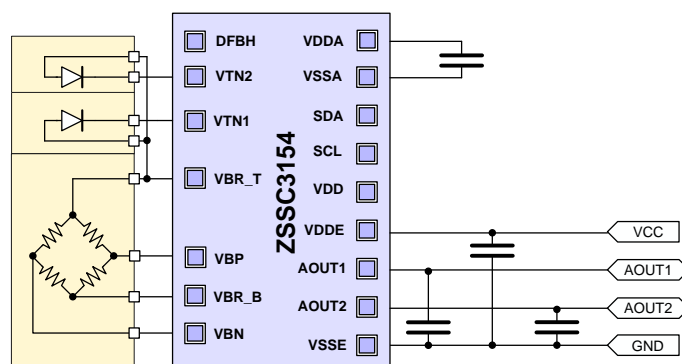
Figure 1. Basic Circuit
