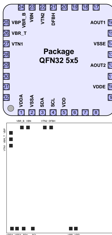
Figure 8. Pin Map and Pad Position of the ZSSC3154
