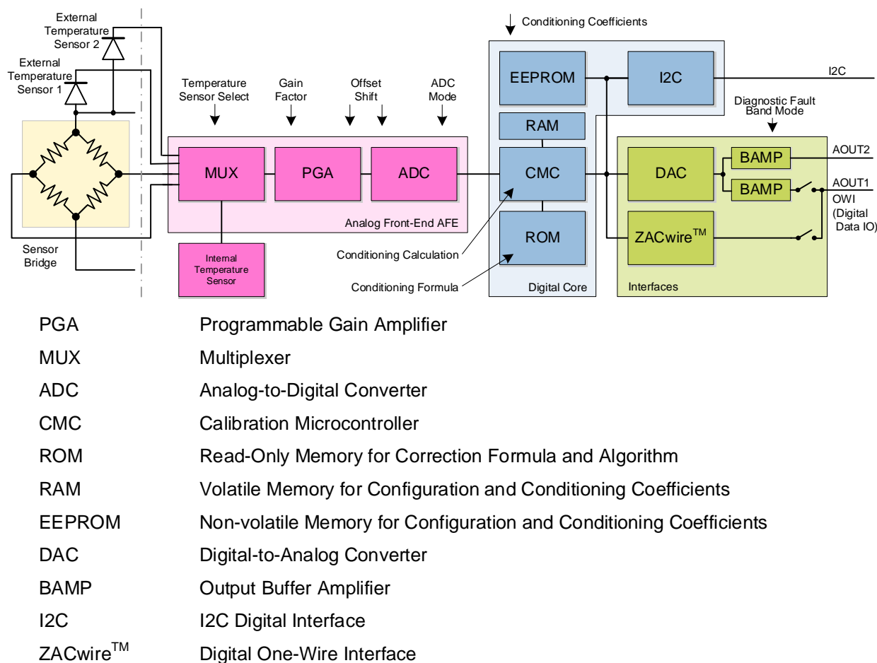
Figure 3. Block Diagram of the ZSSC3154
