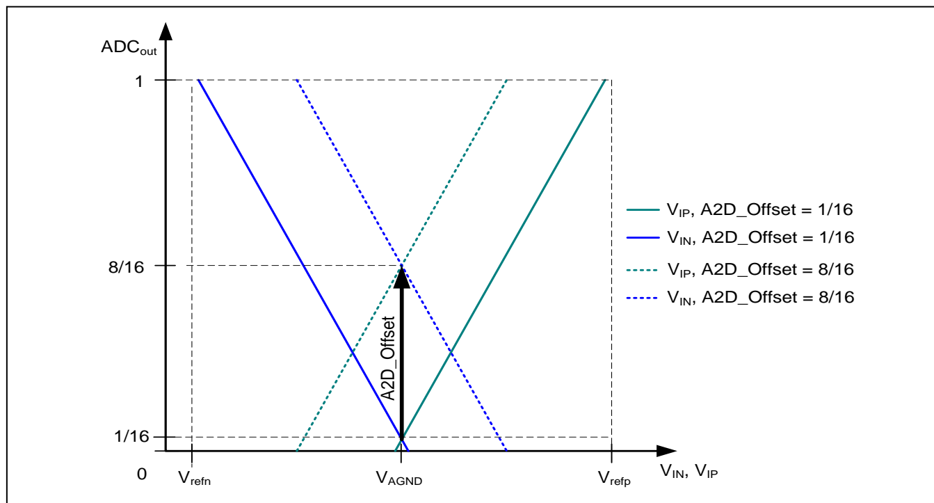
Figure 2.2 ADC Offset
