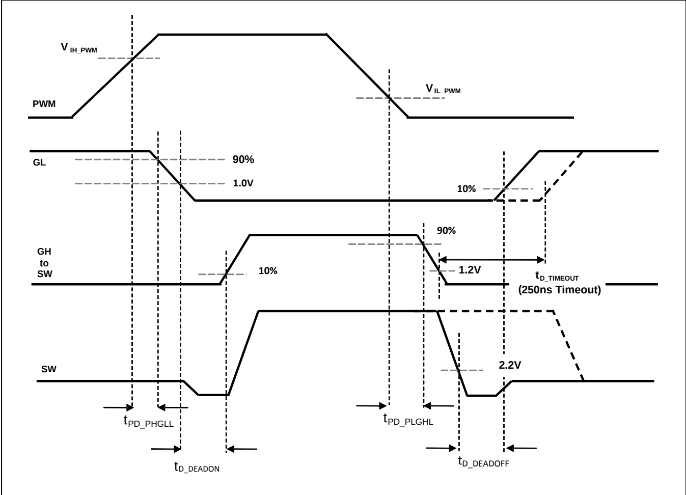
Figure 2.6 PWM Timing
