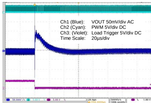
Figure 4-36 20 to 5A Load Step – Max. Capacitance
