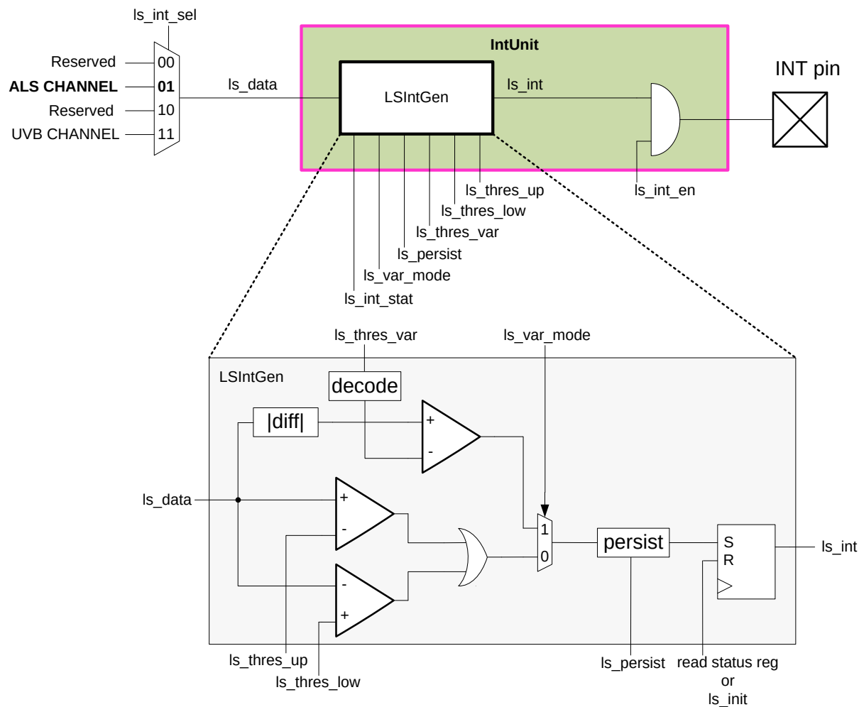
Figure 3.5 Interrupt Unit
