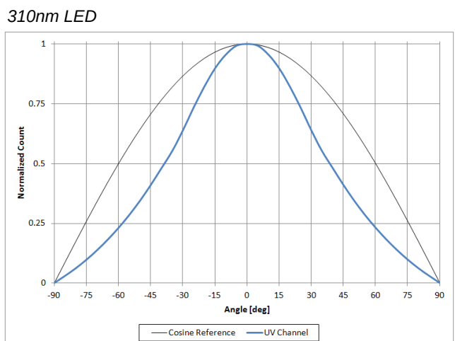
Figure 2.9 UVBS Sensitivity vs. Angle of Incidence
