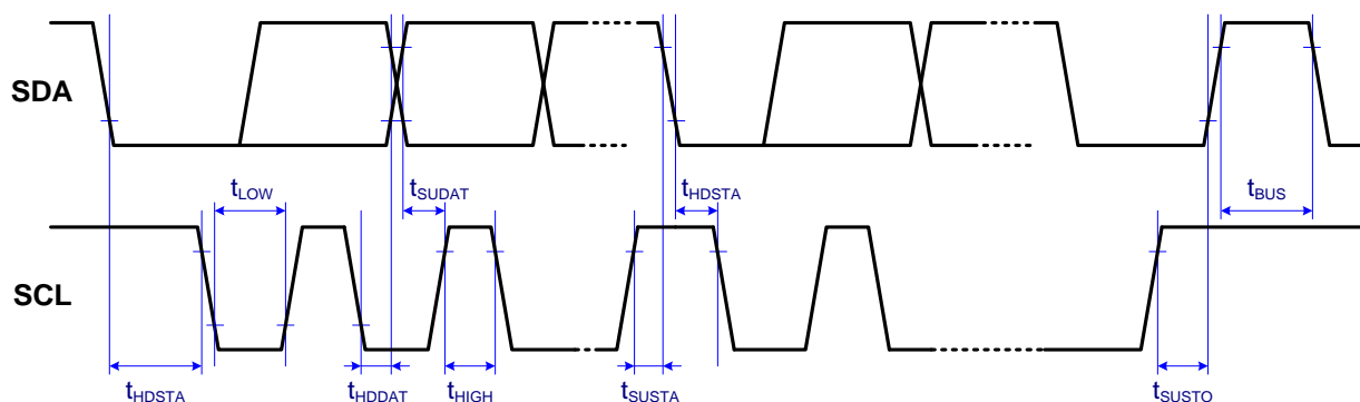
Figure 15. Bus Timing
