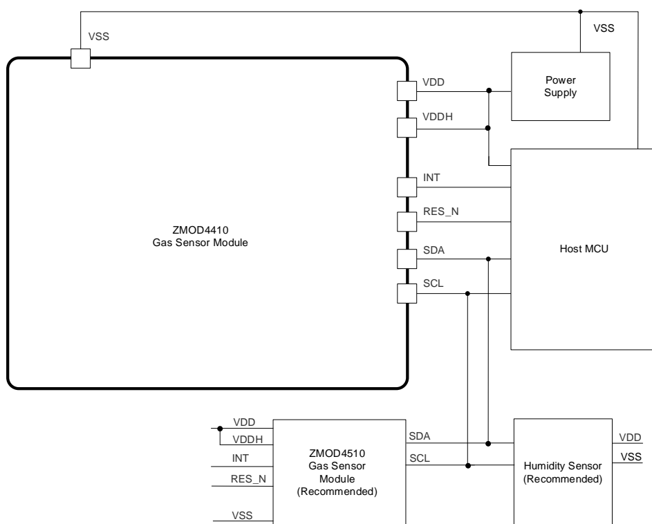
Figure 2. Application Circuit
