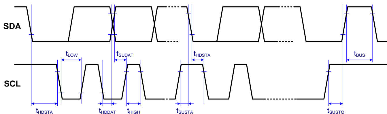
Figure 15. Bus Timing
