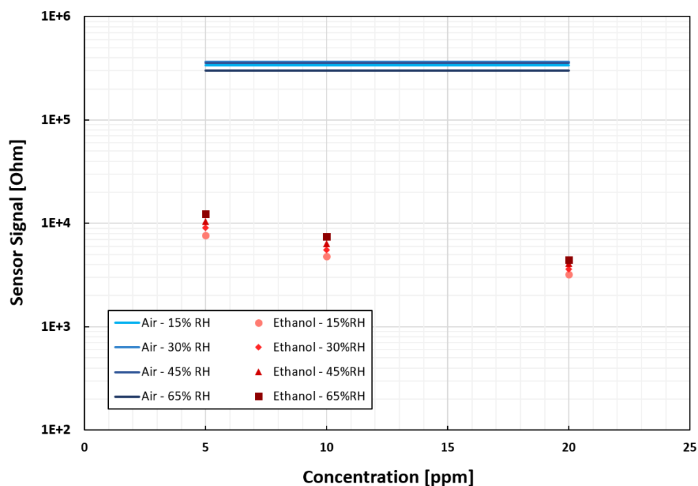
Figure 7. Humidity Influence at Three Different VOC Concentrations
