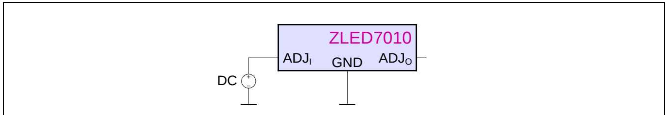
Figure 2.2 External DC Control Voltage at ADJ i Pin
