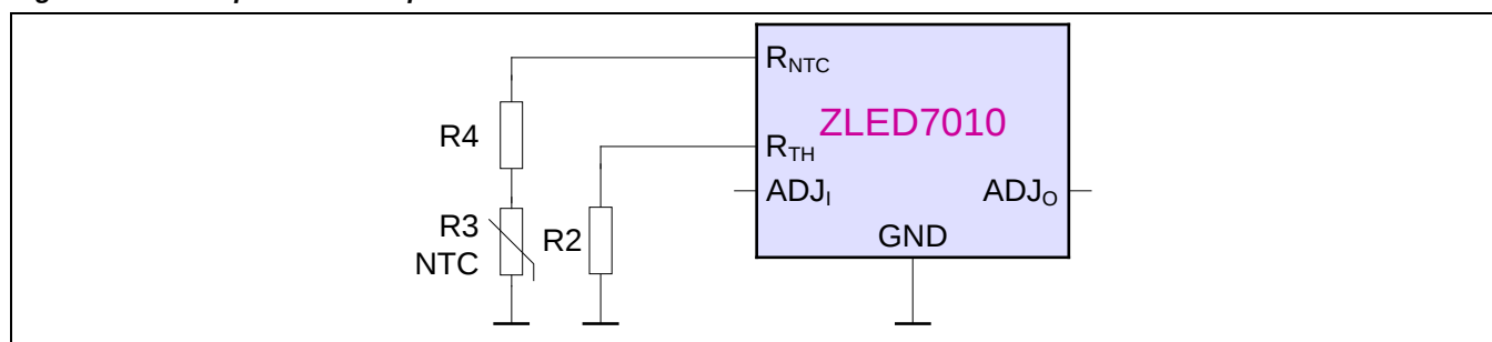
Figure 4.1 Temperature Compensation
