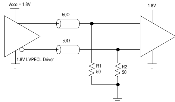
Figure 6. 1.8V LVPECL Driver Termination Example
