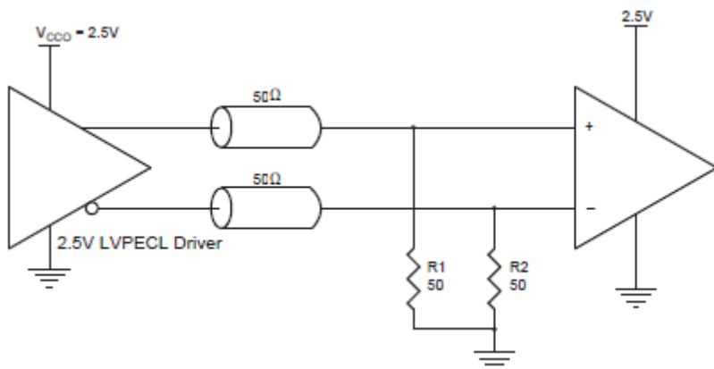
Figure 9. 2.5V LVPECL Driver Termination Example
