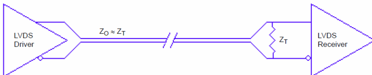
Figure 9. Standard LVDS Termination
