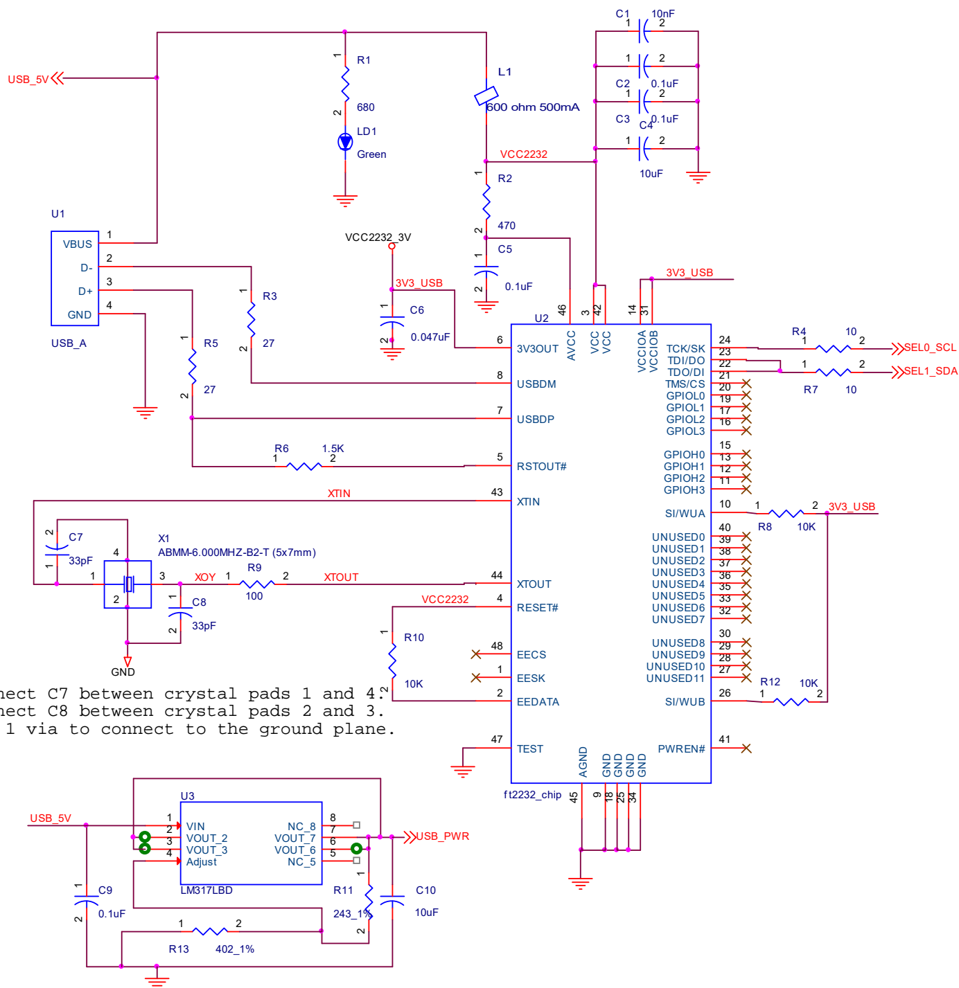
Figure 12. 5P49V6965/6975 Programmer Board Schematics – page 2
