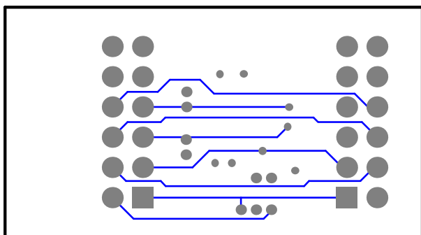
Figure 11. Bottom Layer
