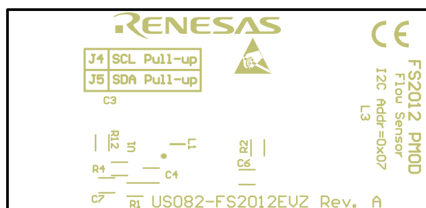
Figure 9. Silkscreen Bottom Layer
