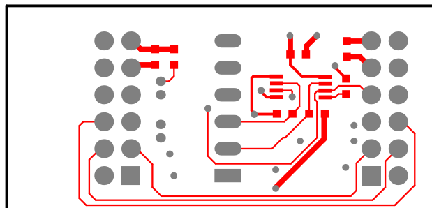
Figure 5. Top Layer
