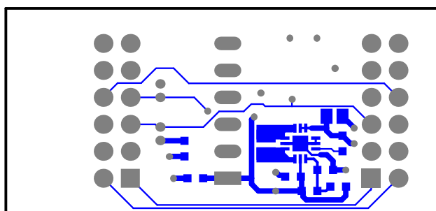
Figure 8. Bottom Layer
