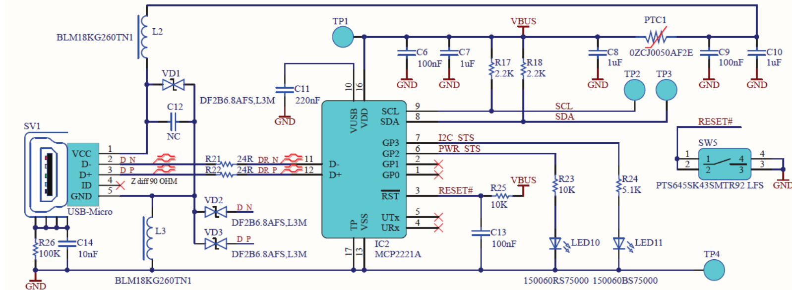
Figure 15: USB-I 2 C Bridge
